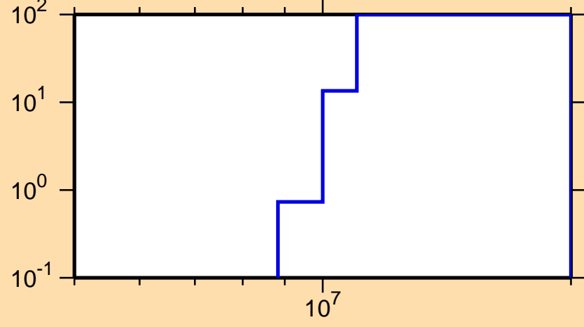
\Delta\sigma/\sigma vs. E for ^{71}\text{Ni}(n,p)
