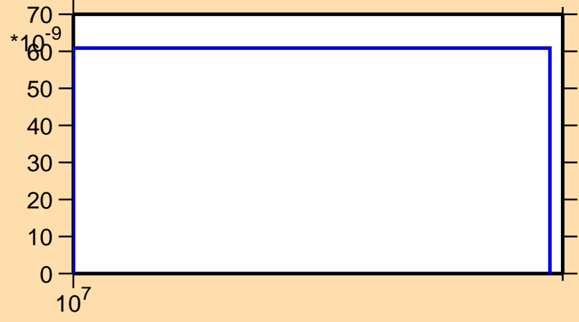
\sigma vs. E for ^{71}\text{Ni}(n,np)
