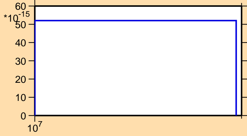
\sigma vs. E for ^{71}\text{Ni}(n,nt)
