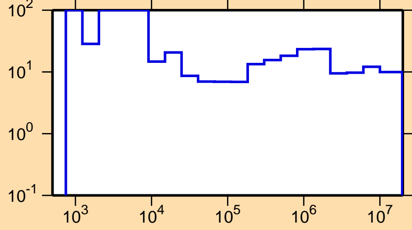
\Delta\sigma/\sigma vs. E for ^{71}\text{Ni}(n,\text{tot.})
