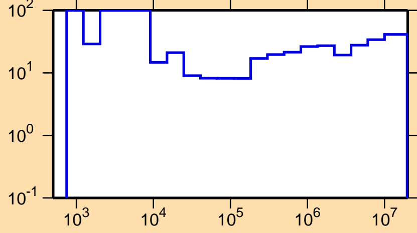
\Delta\sigma/\sigma vs. E for ^{71}\text{Ni}(n,\text{el.})
