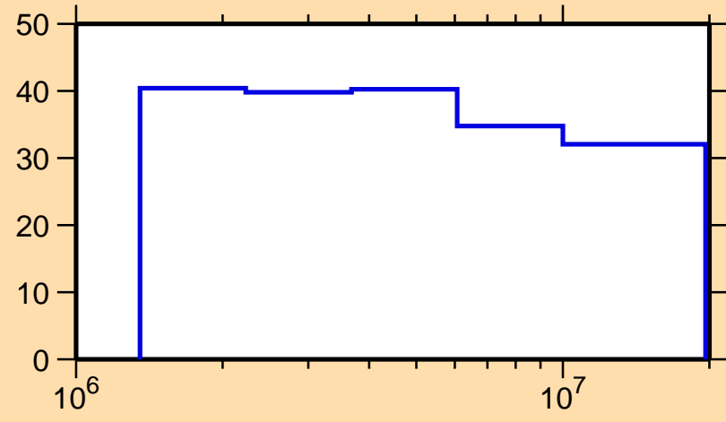
\Delta\sigma/\sigma vs. E for ^{71}\text{Ni}(n,\text{nonel.})
