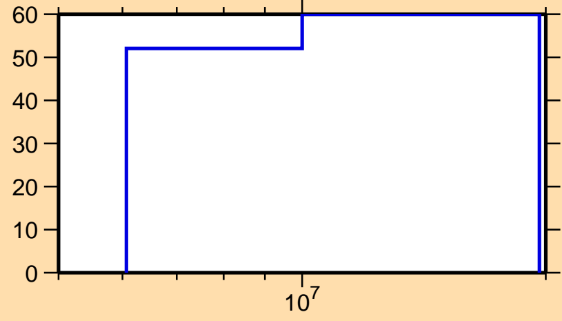
\Delta\sigma/\sigma vs. E for ^{71}\text{Ni}(n,ncont.)
