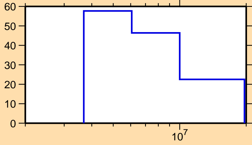
\Delta\sigma/\sigma vs. E for ^{71}\text{Ni}(n,2n)
