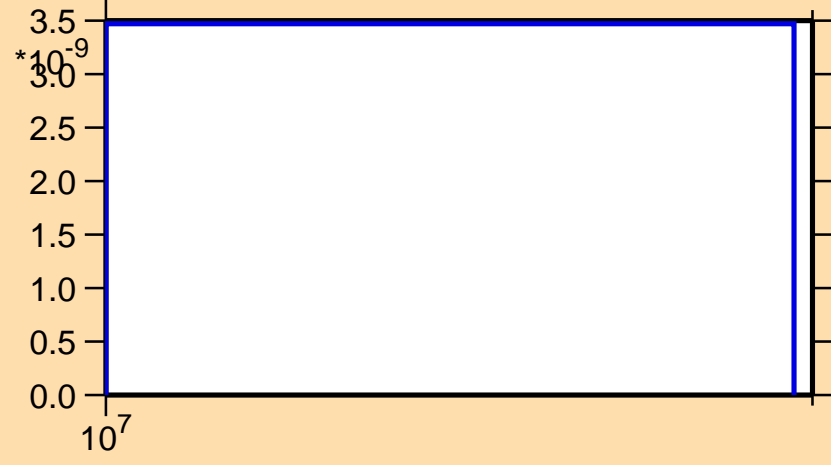
\sigma vs. E for ^{71}\text{Ni}(n,n\alpha)
