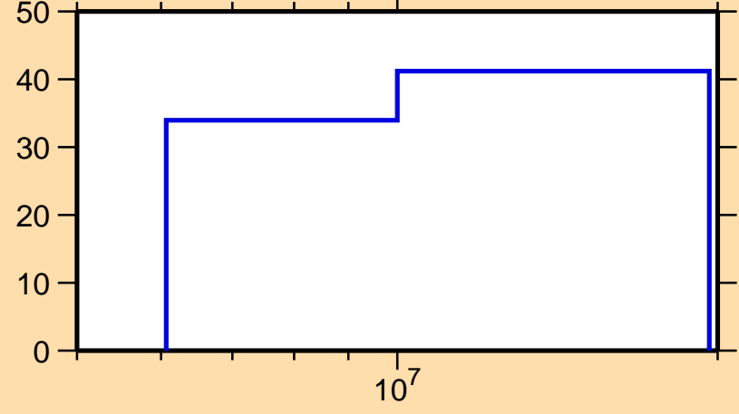
\Delta\sigma/\sigma vs. E for ^{71}\text{Ni}(n,el.)
