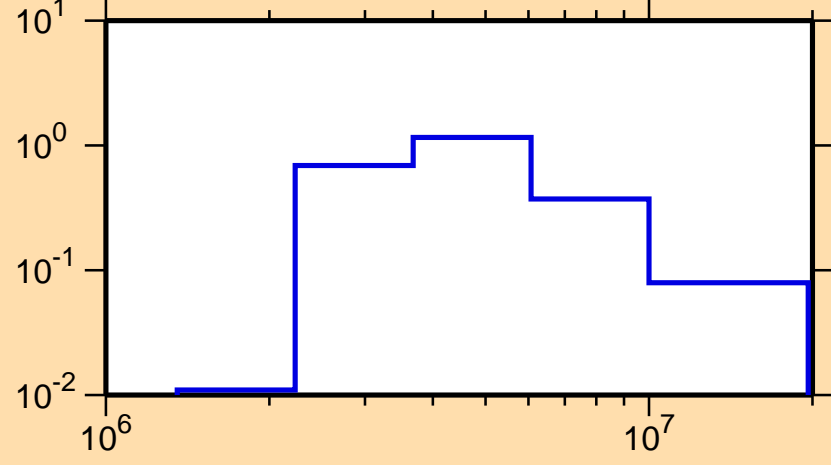
\sigma vs. E for ^{71}\text{Ni}(n,n\text{cont.})
