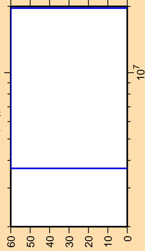
\Delta\sigma/\sigma vs. E for ^{71}\text{Ni}(n,\gamma)
