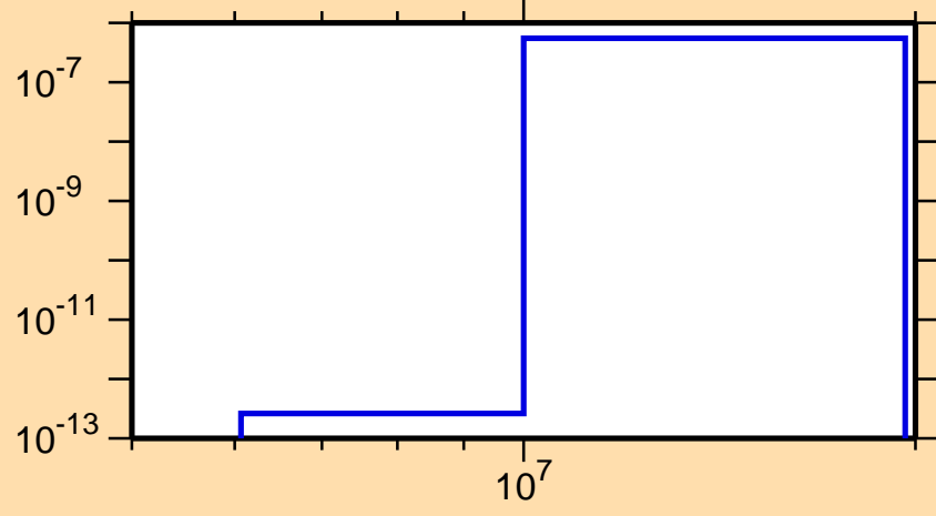
\sigma vs. E for ^{71}\text{Ni}(n,\alpha)
