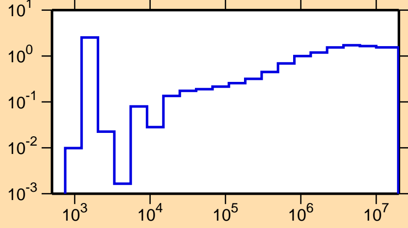
\sigma vs. E for ^{71}\text{Ni}(n,\text{nonel.})
