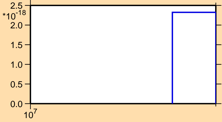
\sigma vs. E for ^{72}\text{Ni}(n,nt)
