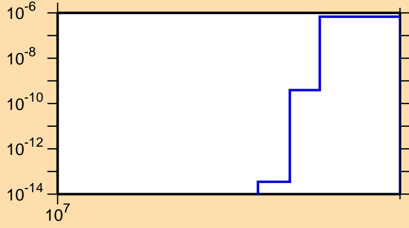
\sigma vs. E for ^{72}\text{Ni}(n,t)
