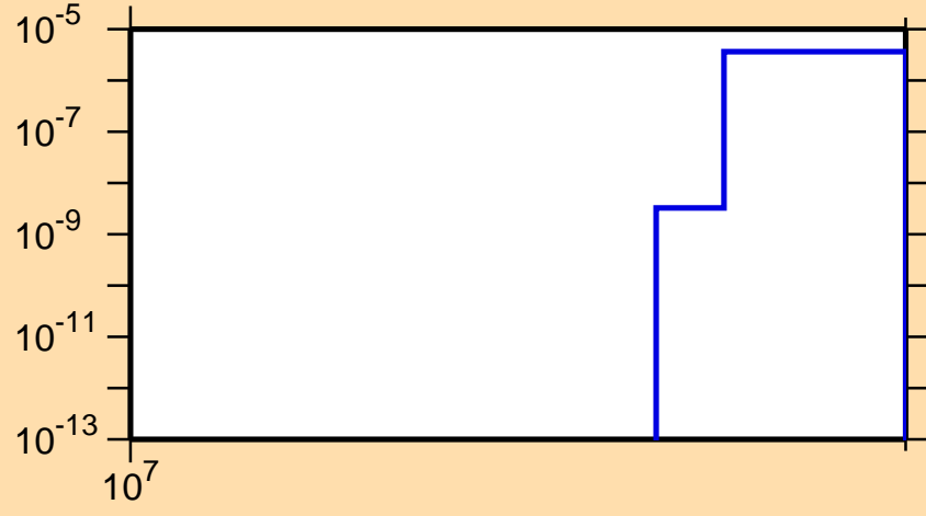
\sigma vs. E for ^{72}\text{Ni}(n,d)
