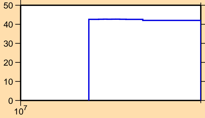
\Delta\sigma/\sigma vs. E for ^{72}\text{Ni}(n,n\text{cont.})
