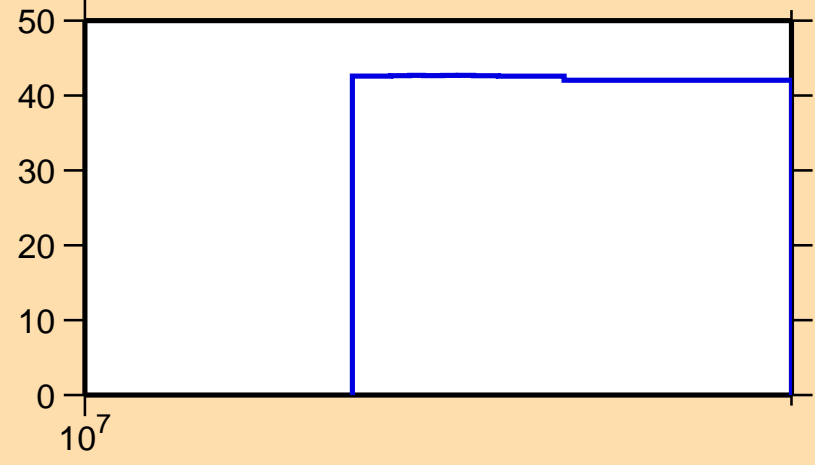
\Delta\sigma/\sigma vs. E for ^{72}\text{Ni}(n,ncont.)
