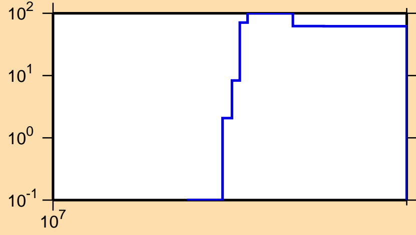
\Delta\sigma/\sigma vs. E for ^{72}\text{Ni}(n,p)
