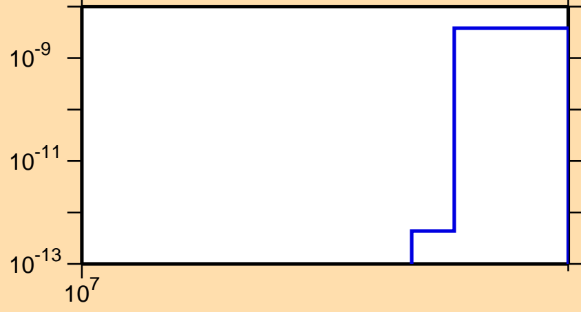
\sigma vs. E for ^{72}\text{Ni}(n,n\alpha)
