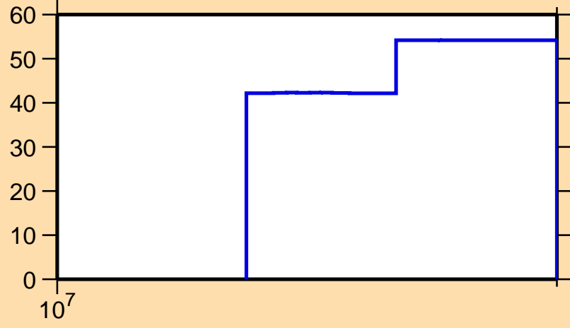
\Delta\sigma/\sigma vs. E for ^{72}\text{Ni}(n,el.)
