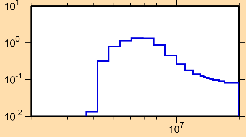
\sigma vs. E for ^{72}\text{Ni}(n,n\text{cont.})
