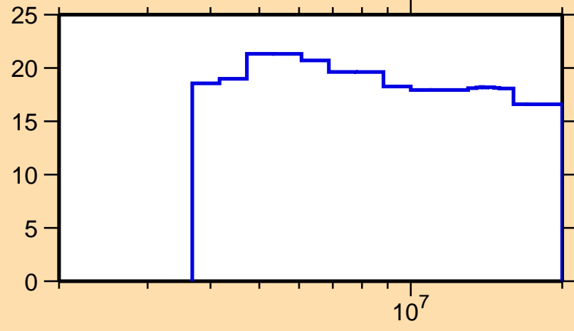
\Delta\sigma/\sigma vs. E for ^{72}\text{Ni}(n,\text{nonel.})
