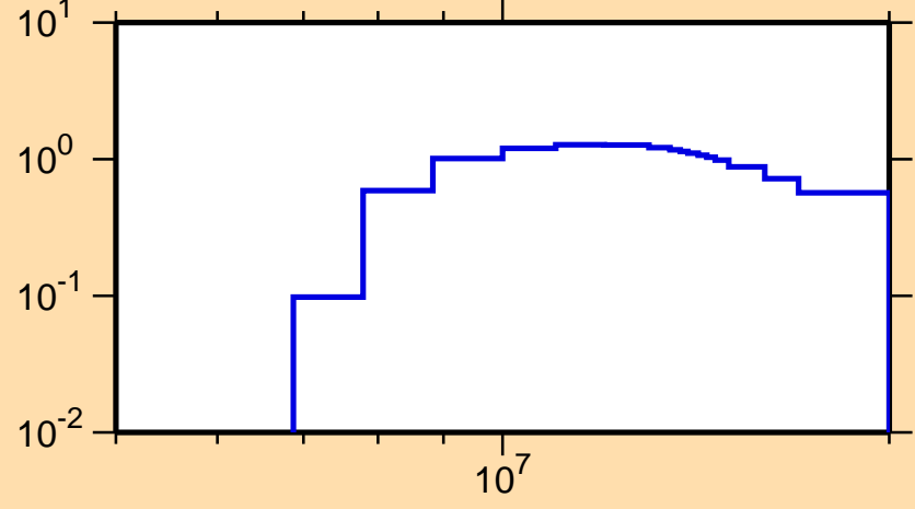
\sigma vs. E for ^{72}\text{Ni}(n,2n)
