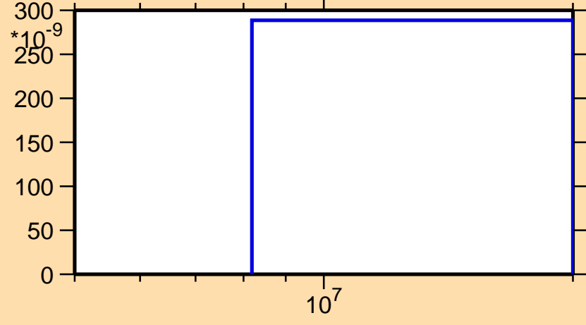
\sigma vs. E for ^{72}\text{Ni}(n,p)
