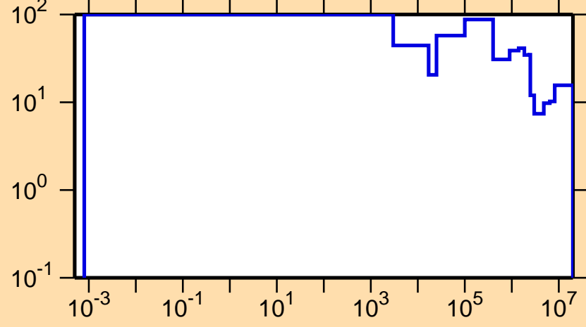
\Delta\sigma/\sigma vs. E for ^{72}\text{Ni}(n,\text{tot.})
