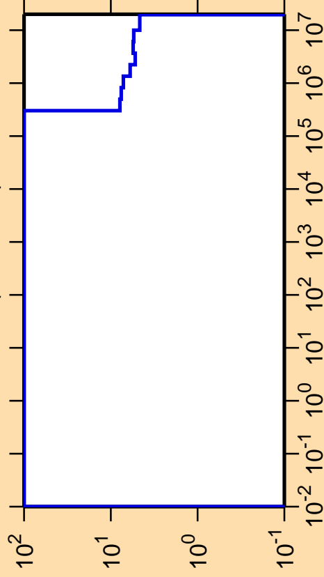
\Delta\sigma/\sigma vs. E for ^{14}\text{O}(n,\text{nonel.})
