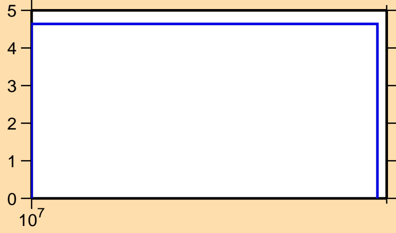
\Delta\sigma/\sigma vs. E for ^{14}\text{O}(n,n\text{onel.})
