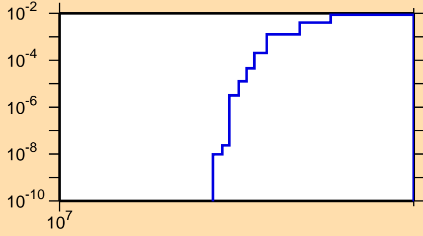
\sigma vs. E for ^{15}\text{O}(n,\text{pd})
