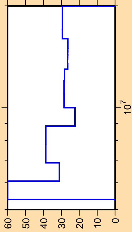
\Delta\sigma/\sigma vs. E for ^{15}\text{O}(n,d)
