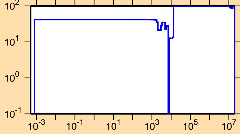
\Delta\sigma/\sigma vs. E for ^{15}\text{O}(n,\gamma)
