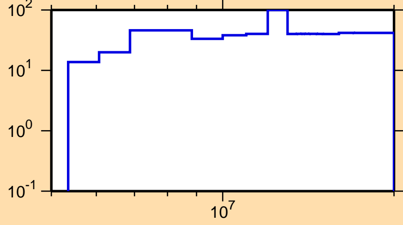
\Delta\sigma/\sigma vs. E for ^{15}\text{O}(n,n_1)
