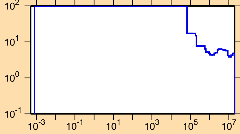
\Delta\sigma/\sigma vs. E for ^{15}\text{O}(n,\text{nonel.})
