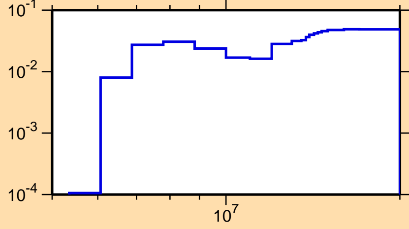
\sigma vs. E for ^{15}\text{O}(n,d)
