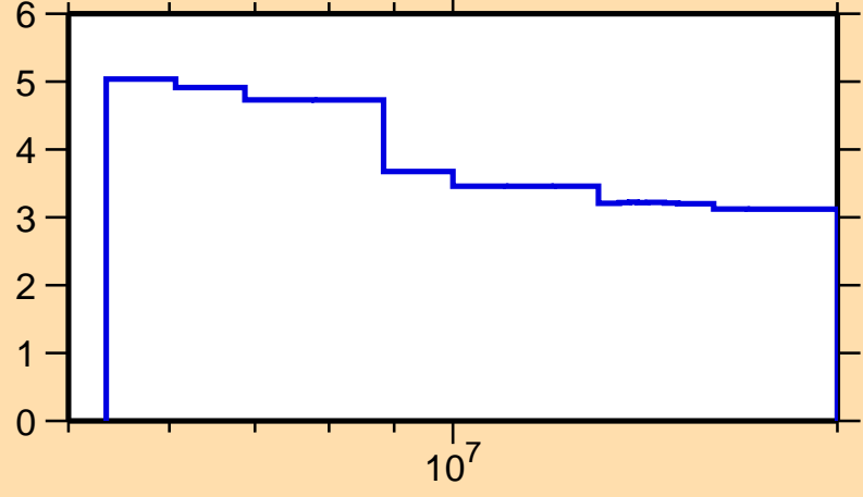
\Delta\sigma/\sigma vs. E for ^{15}\text{O}(n,\text{tot.})
