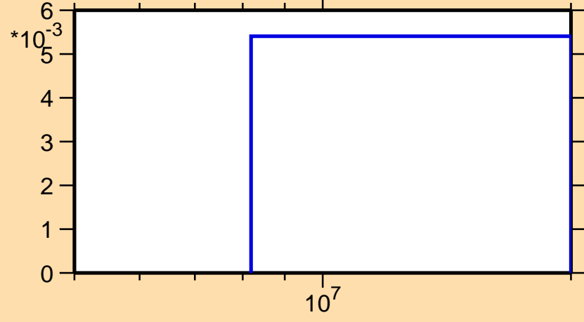
\sigma vs. E for ^{15}\text{O}(n,n\alpha)
