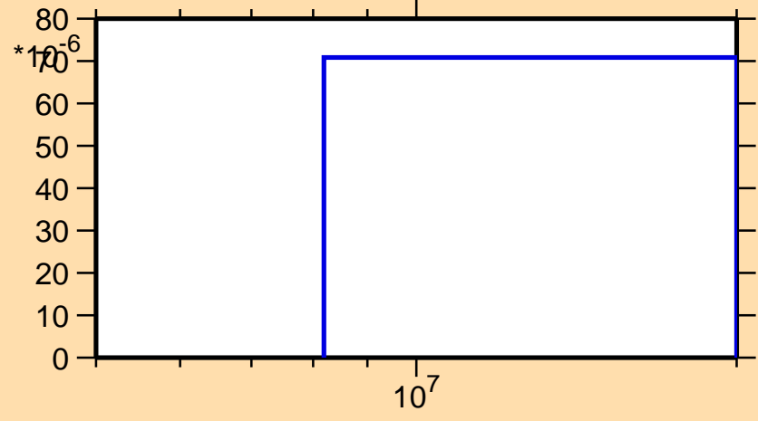
\sigma vs. E for ^{15}\text{O}(n,t)
