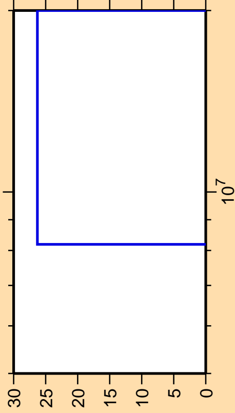
\Delta\sigma/\sigma vs. E for ^{15}\text{O}(n,\text{pd})
