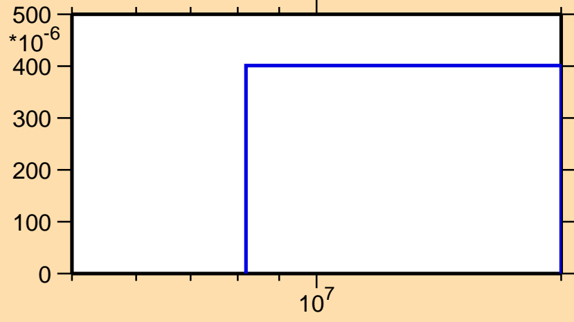
\sigma vs. E for ^{15}\text{O}(n,\text{pd})
