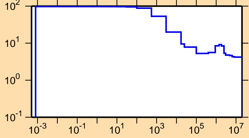
\Delta\sigma/\sigma vs. E for ^{15}\text{O}(n,\text{el.})
