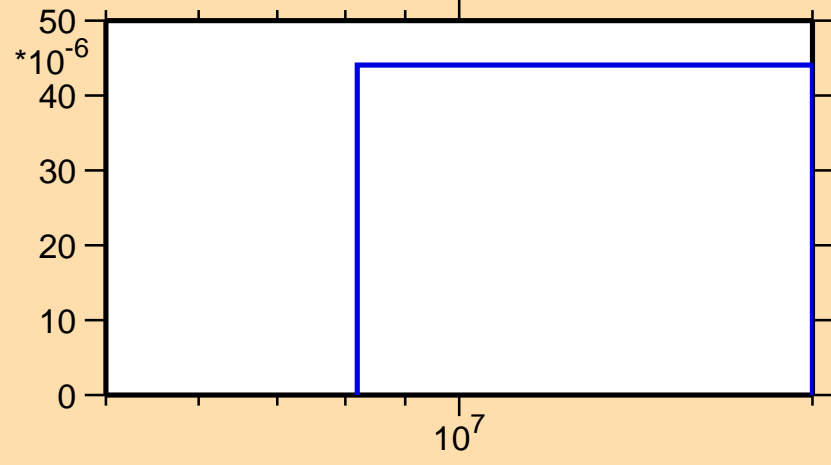
\sigma vs. E for ^{15}\text{O}(n,\text{pt})
