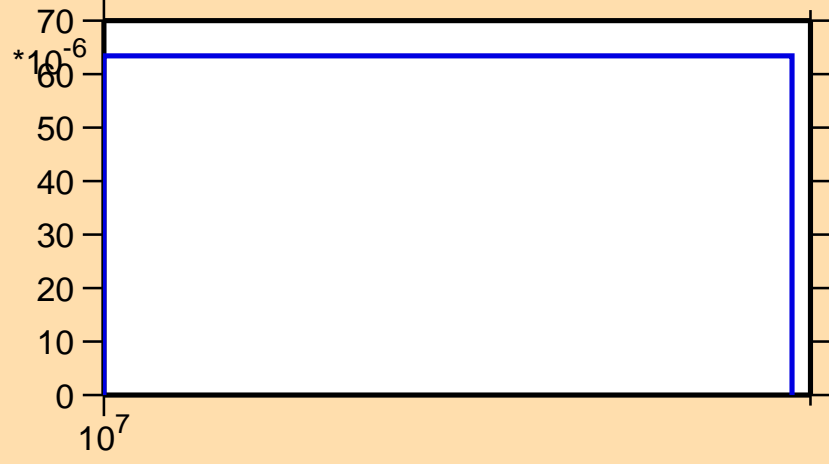
\sigma vs. E for ^{19}\text{O}(n,p)
