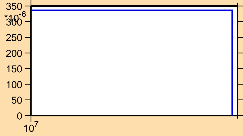
\sigma vs. E for ^{19}\text{O}(n,t)
