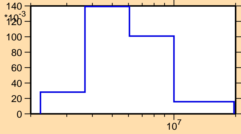
\sigma vs. E for ^{19}\text{O}(n,n_4)
