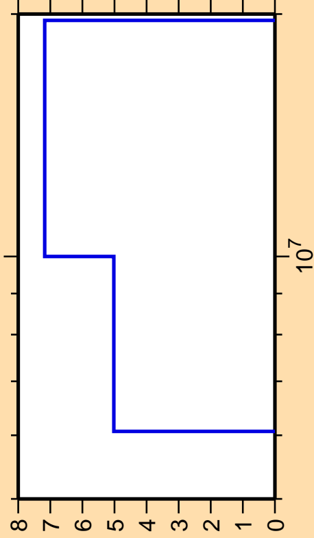
\Delta\sigma/\sigma vs. E for ^{19}\text{O}(n,2n)
