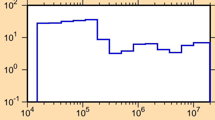
\Delta\sigma/\sigma vs. E for ^{19}\text{O}(n,\text{el.})
