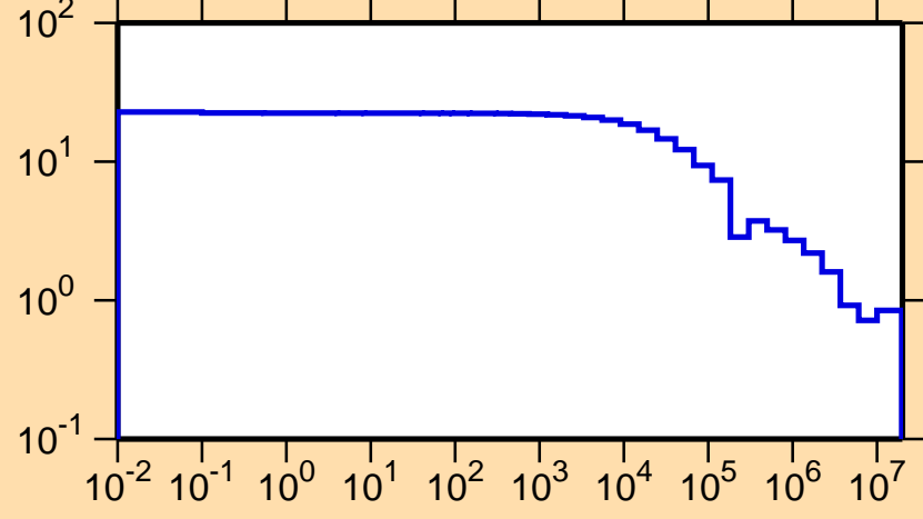
\sigma vs. E for ^{19}\text{O}(n,\text{el.})
