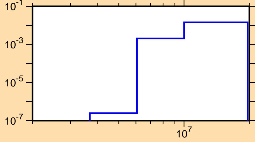
\sigma vs. E for ^{19}\text{O}(n,\alpha)
