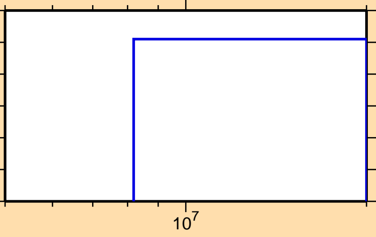
\sigma vs. E for ^{19}\text{O}(n,p)
