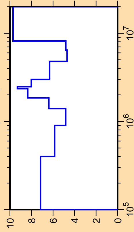
\sigma vs. E for ^{19}\text{O}(n,\text{inel.})
