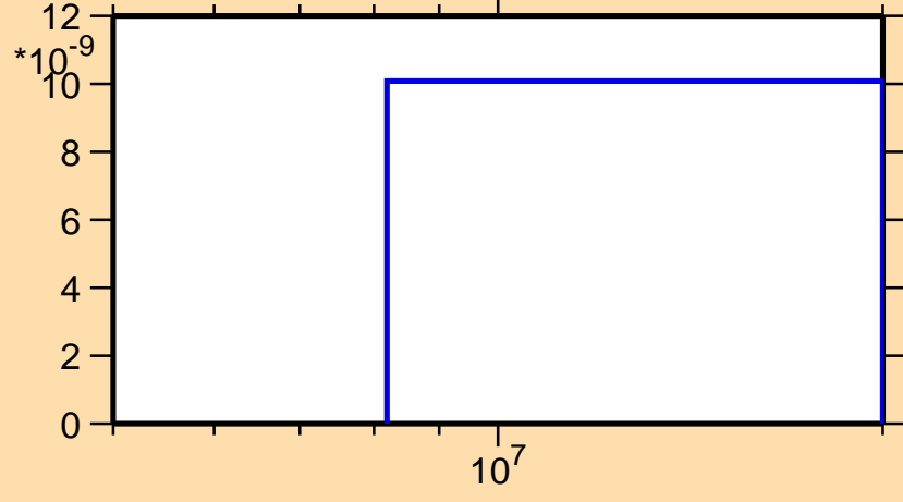
\sigma vs. E for ^{19}\text{O}(n,\text{nd})
