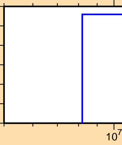
\sigma vs. E for ^{19}\text{O}(n,d)
