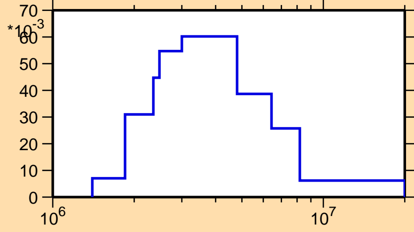
\sigma vs. E for ^{19}\text{O}(n,n_2)
