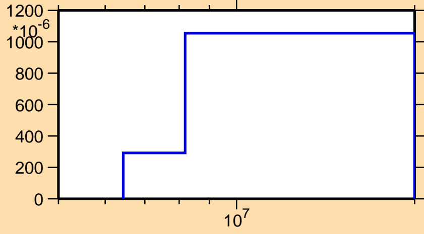
\sigma vs. E for ^{19}\text{O}(n,n\text{cont.})
