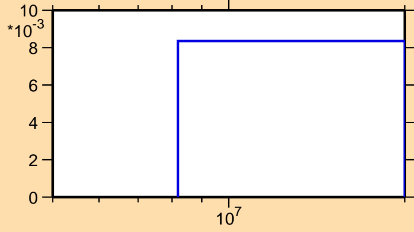
\sigma vs. E for ^{19}\text{O}(n,n\alpha)
