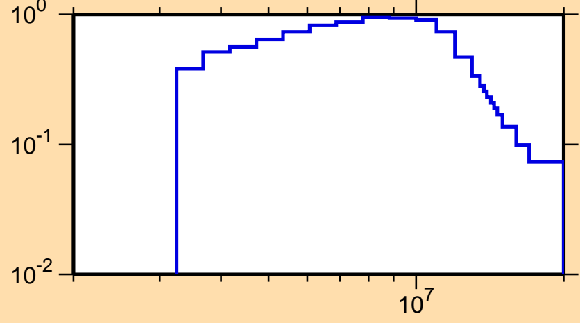
\sigma vs. E for ^{20}\text{O}(n,\text{inel.})
