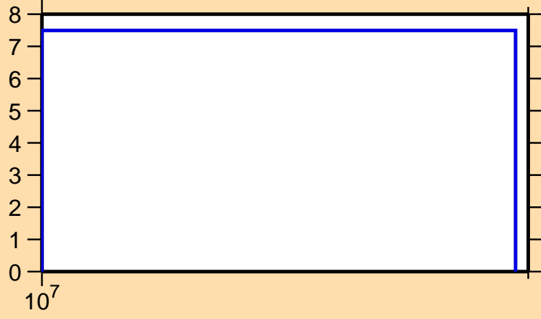
\Delta\sigma/\sigma vs. E for ^{20}\text{O}(n,incl.)
