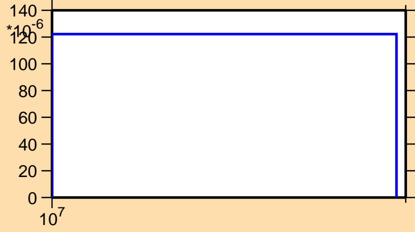
\sigma vs. E for ^{20}\text{O}(n,n\alpha)
