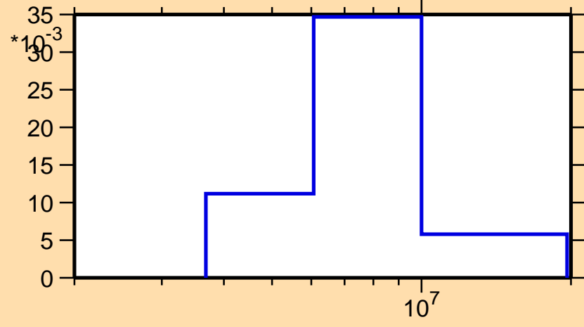
\sigma vs. E for ^{20}\text{O}(n,n_4)
