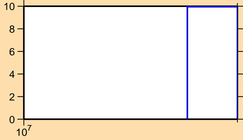
\Delta\sigma/\sigma vs. E for ^{21}\text{O}(n,el.)
