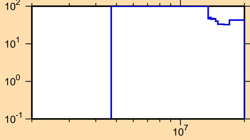
\Delta\sigma/\sigma vs. E for ^{21}\text{O}(n,n\text{cont.})
