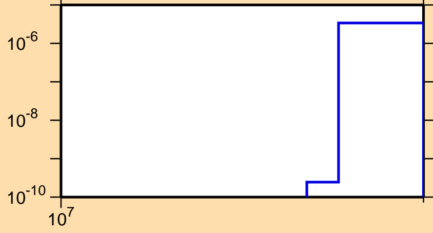
\sigma vs. E for ^{21}\text{O}(n,n\alpha)
