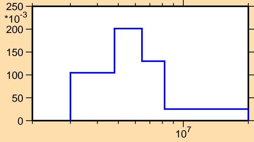
\sigma vs. E for ^{21}\text{O}(n,n_3)
