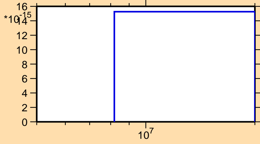
\sigma vs. E for ^{21}\text{O}(n,d)
