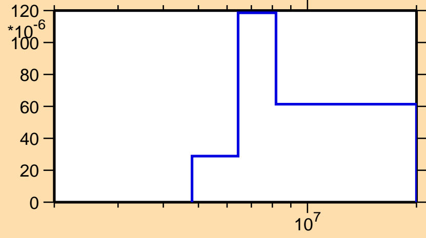
\sigma vs. E for ^{21}\text{O}(n,n\text{cont.})
