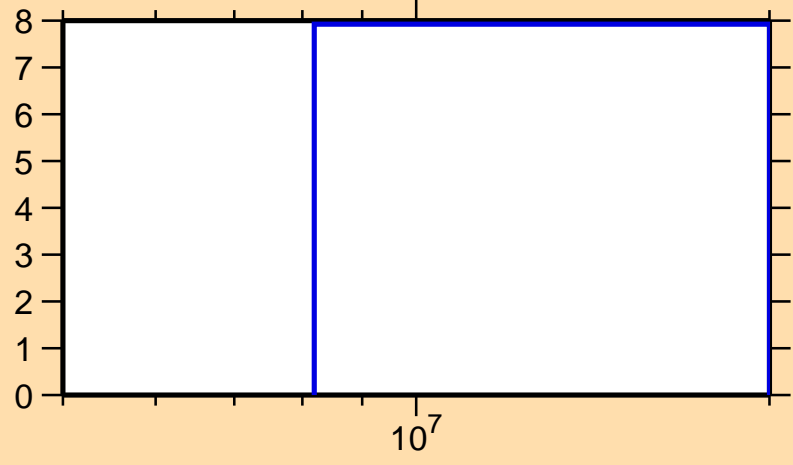
\Delta\sigma/\sigma vs. E for ^{21}\text{O}(n,el.)
