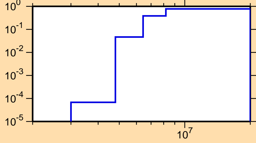
\sigma vs. E for ^{21}\text{O}(n,2n)
