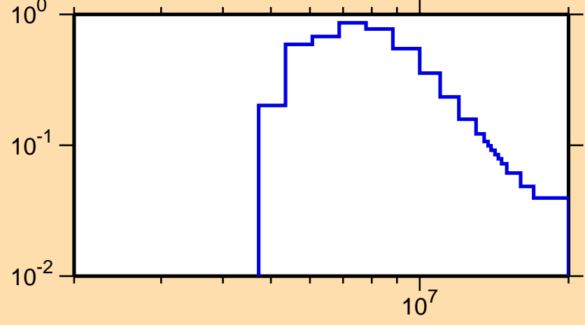
\sigma vs. E for ^{22}\text{O}(n,\text{inel.})
