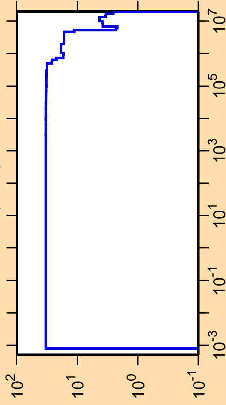
\Delta\sigma/\sigma vs. E for ^{22}\text{O}(n,\text{el.})
