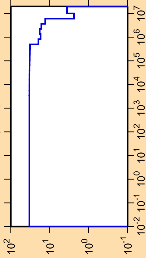
\Delta\sigma/\sigma vs. E for ^{22}\text{O}(n,\text{el.})
