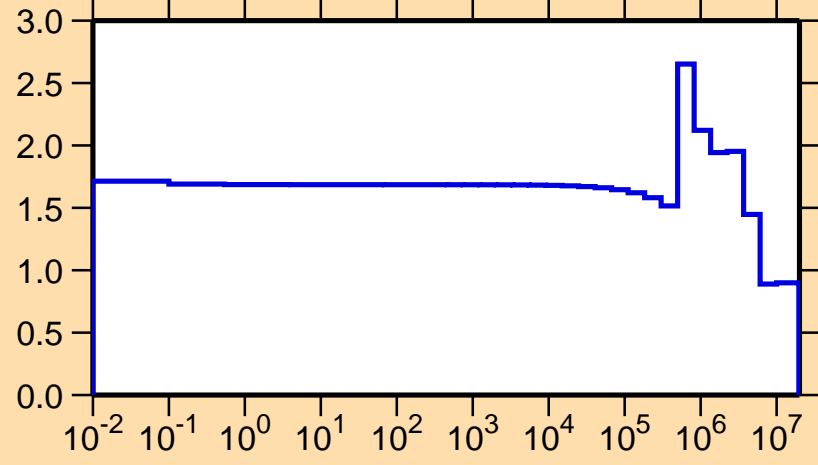
\sigma vs. E for ^{22}\text{O}(n,\text{el.})
