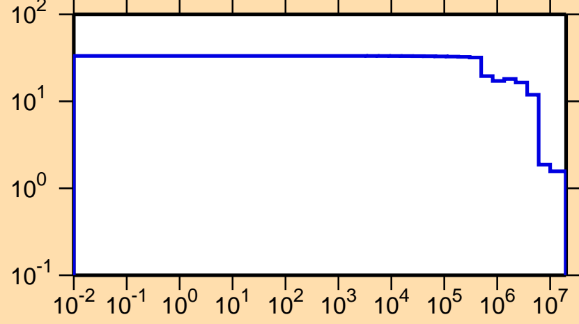
\Delta\sigma/\sigma vs. E for ^{22}\text{O}(n,\text{tot.})
