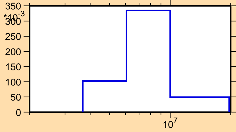
\sigma vs. E for ^{22}\text{O}(n,n_1)
