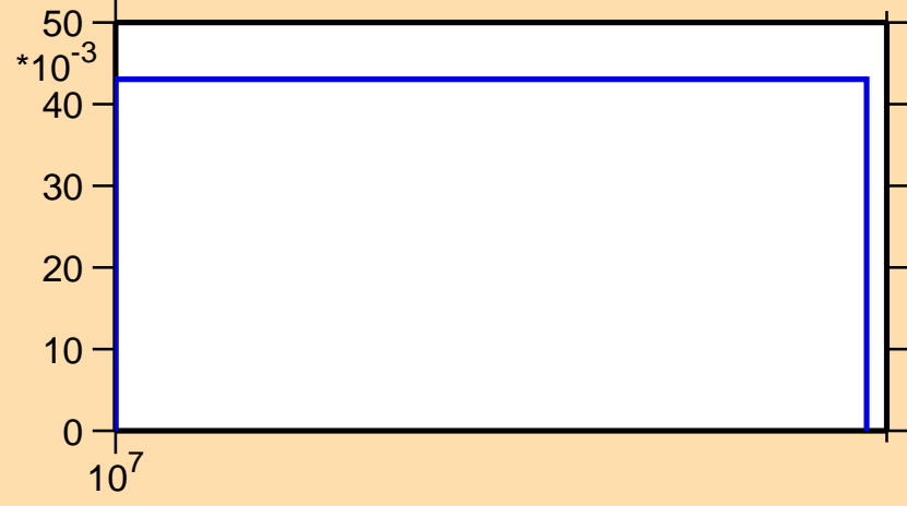
\sigma vs. E for ^{22}\text{O}(n,3n)
