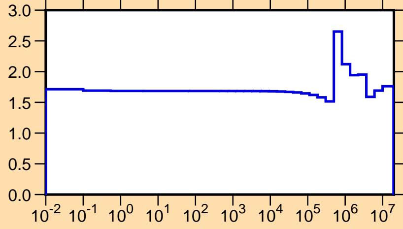
\sigma vs. E for ^{22}\text{O}(n,\text{tot.})
