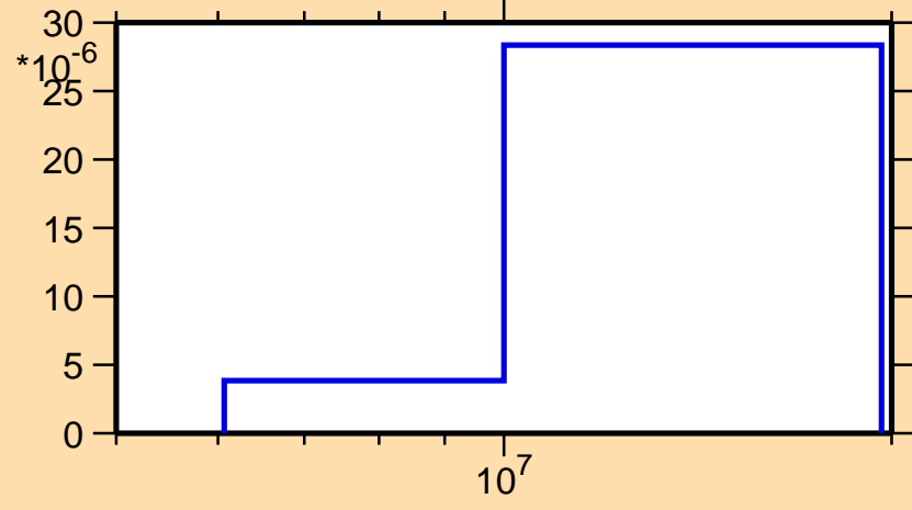
\sigma vs. E for ^{22}\text{O}(n,n\text{cont.})
