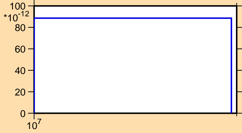
\sigma vs. E for ^{22}\text{O}(n,\alpha)
