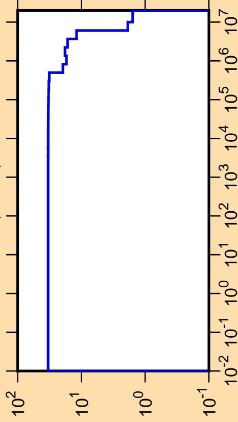
\Delta\sigma/\sigma vs. E for ^{22}\text{O}(n,\text{tot.})
