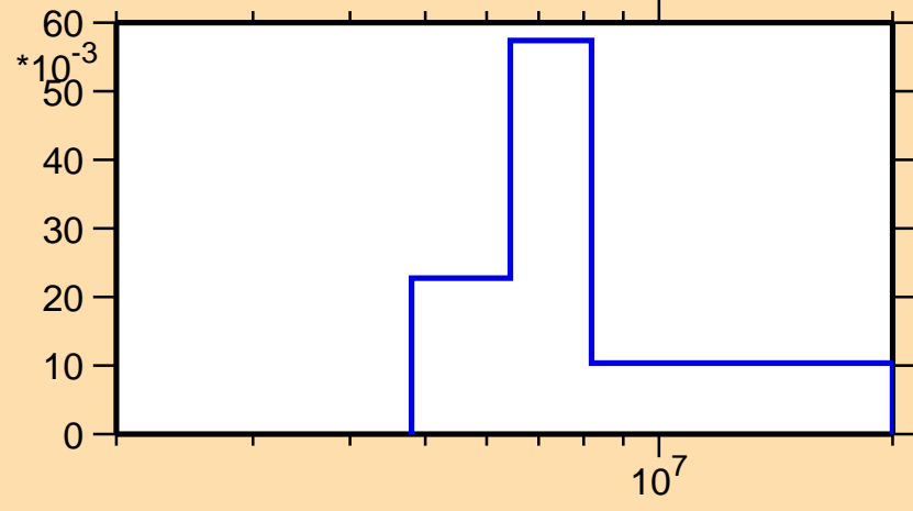
\sigma vs. E for ^{22}\text{O}(n,n_3)
