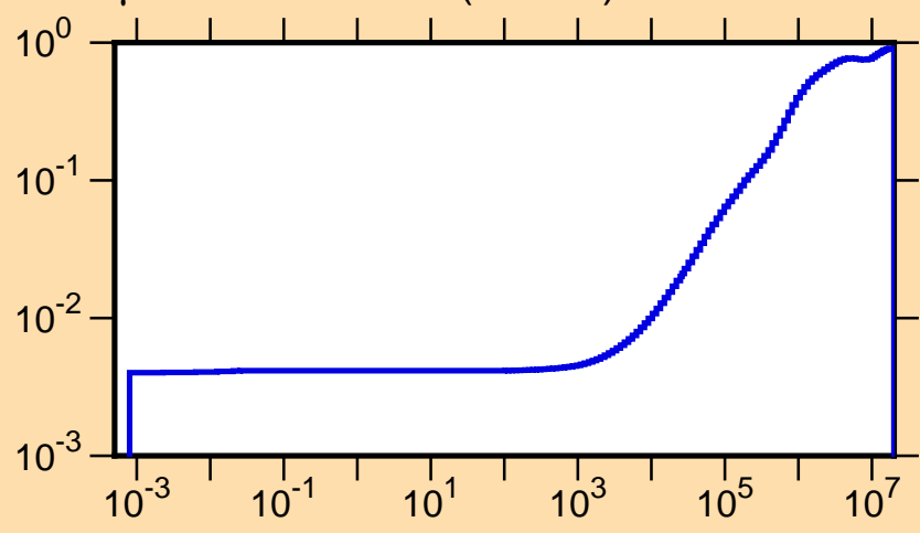
\mu vs. E for ^{168}\text{Os}(\text{mt251})
