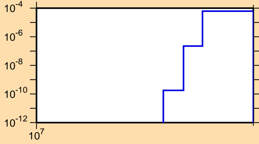
\sigma vs. E for ^{168}\text{Os}(n,2np)
