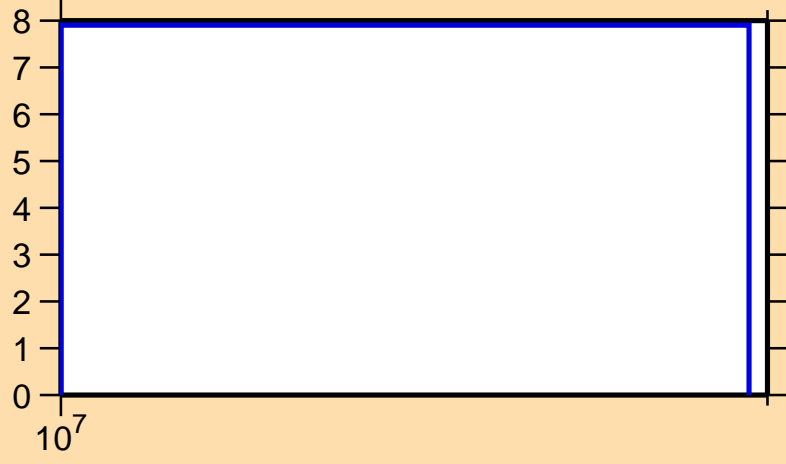
\Delta\sigma/\sigma vs. E for ^{168}\text{Os}(n,\text{el.})
