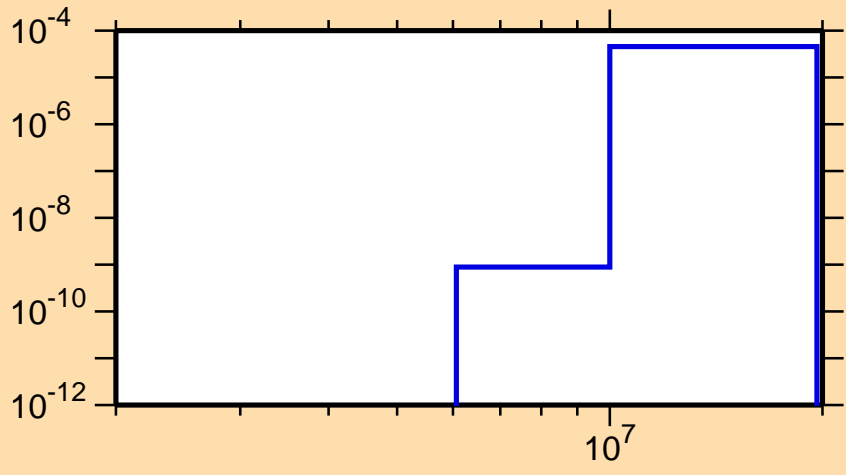
\sigma vs. E for ^{168}\text{Os} (mt 45)
