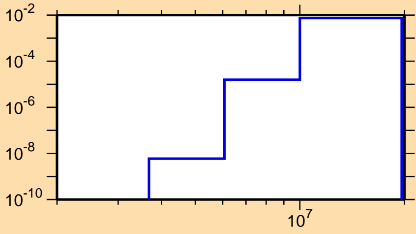
\sigma vs. E for ^{168}\text{Os}(n,d)
