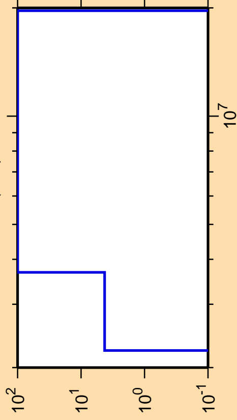
\Delta\sigma/\sigma vs. E for ^{168}\text{Os}(n,d)
