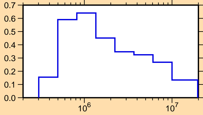
\sigma vs. E for ^{168}\text{Os}(n,n_1)
