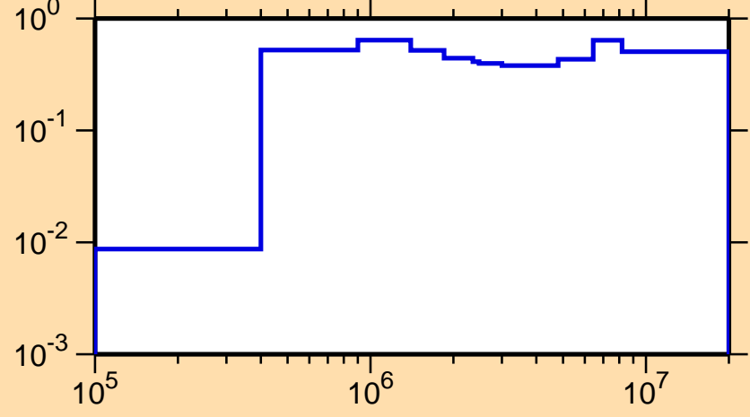
\sigma vs. E for ^{168}\text{Os}(n,\text{inel.})
