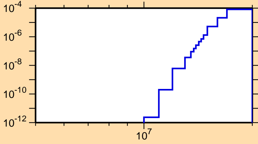
\sigma vs. E for ^{169}\text{Os}(n,\text{pt})
