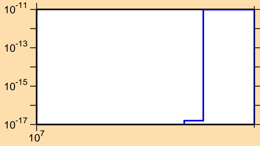
\sigma vs. E for ^{169}\text{Os}(n,nt)
