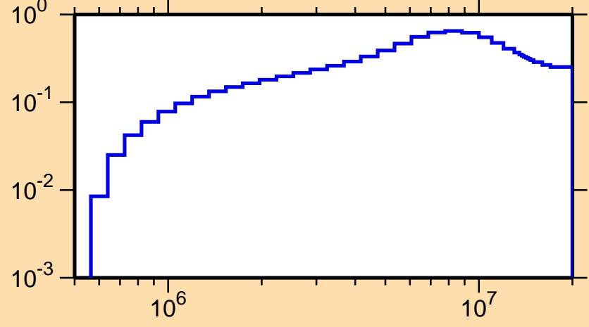
\sigma vs. E for ^{169}\text{Os}(n,n\text{cont.})
