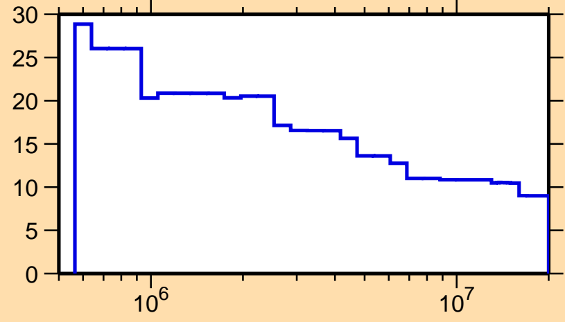
\Delta\sigma/\sigma vs. E for ^{169}\text{Os}(n,n\text{onel.})
