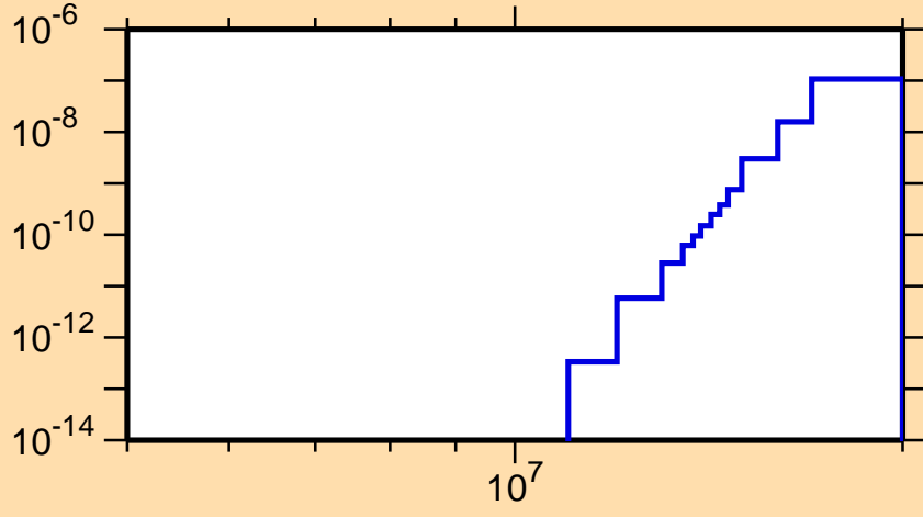
\sigma vs. E for ^{169}\text{Os} (mt 34)
