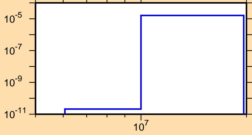
\sigma vs. E for ^{169}\text{Os}(n,\text{pd})
