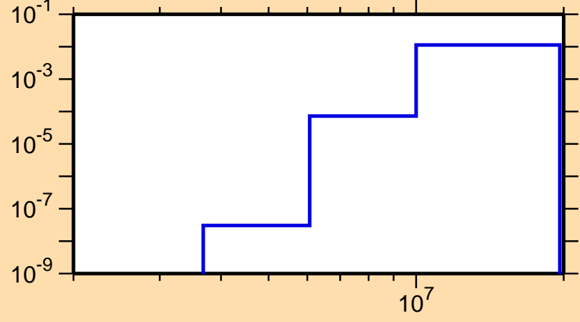
\sigma vs. E for ^{169}\text{Os}(n,d)
