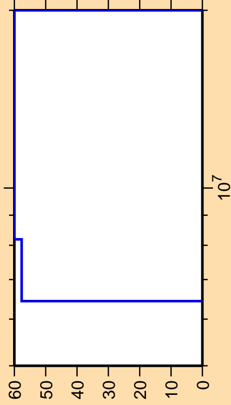
\Delta\sigma/\sigma vs. E for ^{169}\text{Os} (mt 45)
