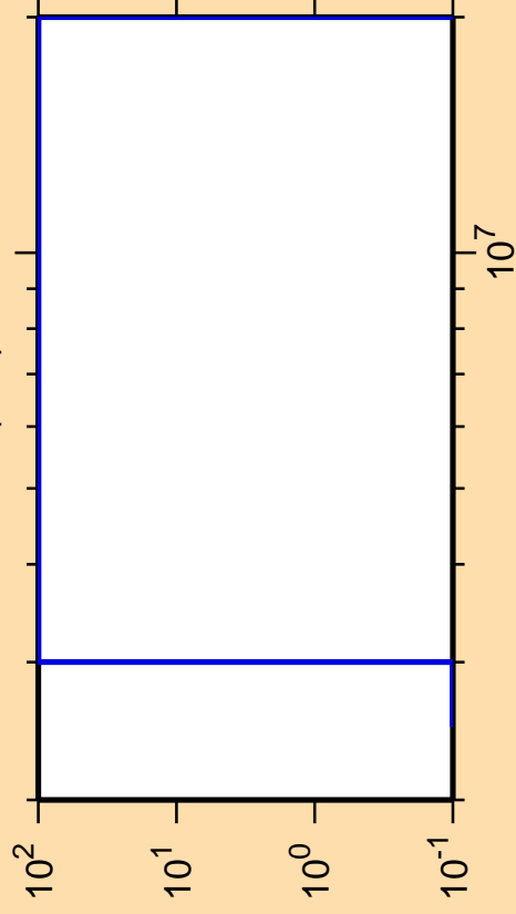
\Delta\sigma/\sigma vs. E for ^{169}\text{Os}(n,d)
