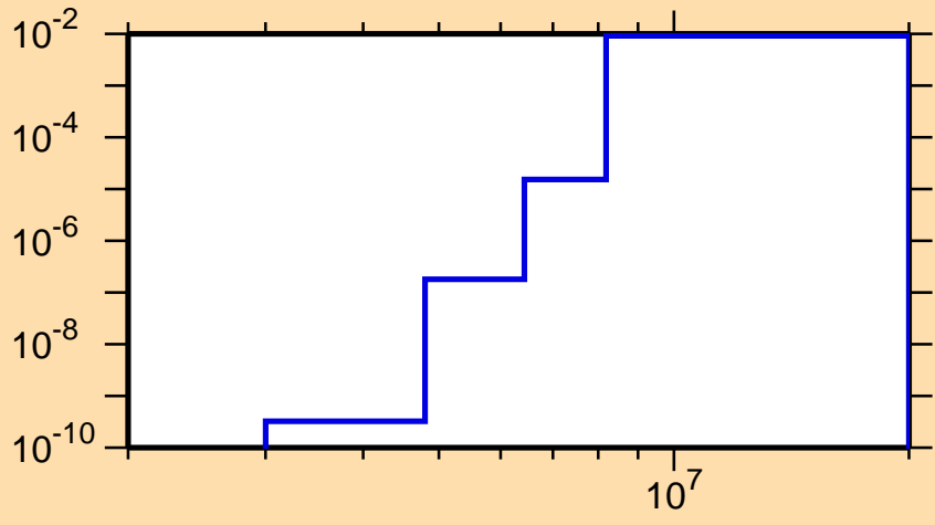
\sigma vs. E for ^{169}\text{Os}(n,d)
