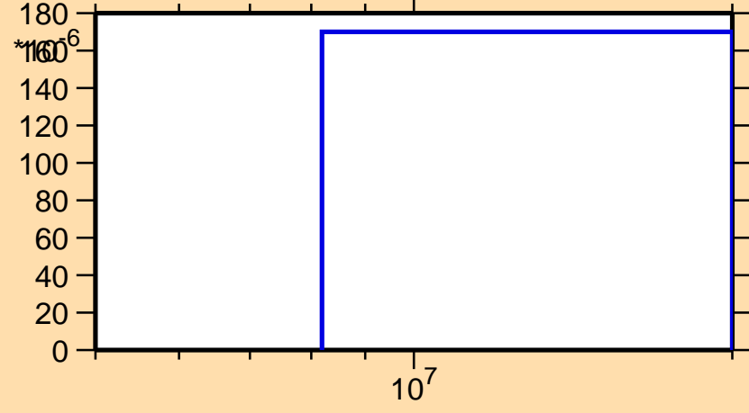
\sigma vs. E for ^{169}\text{Os}(n,2np)
