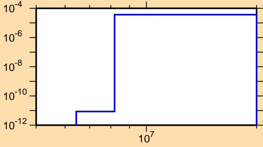
\sigma vs. E for ^{169}\text{Os} (mt 45)
