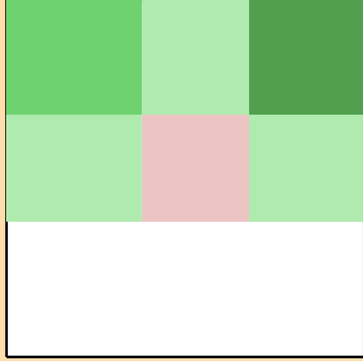
\Delta\sigma/\sigma vs. E for ^{170}\text{Os}(n,\text{nonel.})
