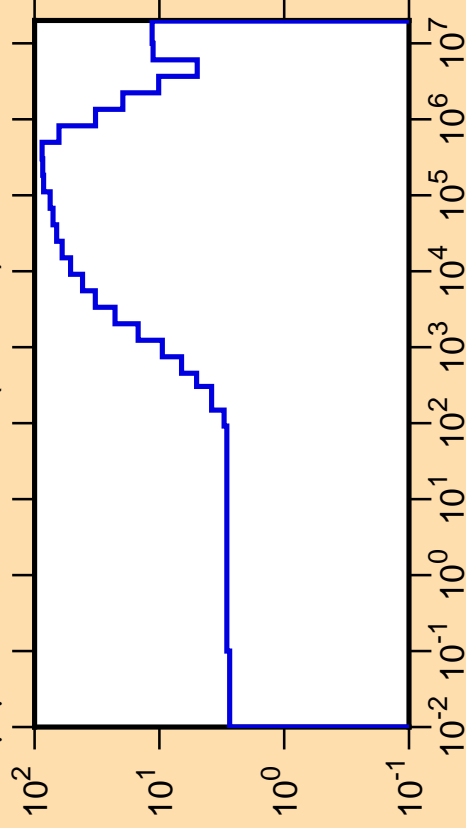
\Delta\mu/\mu vs. E for ^{170}\text{Os}(\text{mt251})
