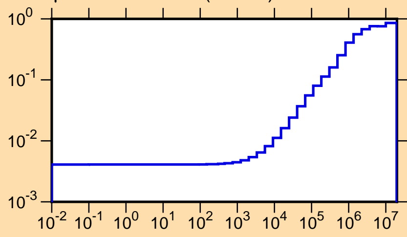
\mu vs. E for ^{170}\text{Os}(\text{mt251})
