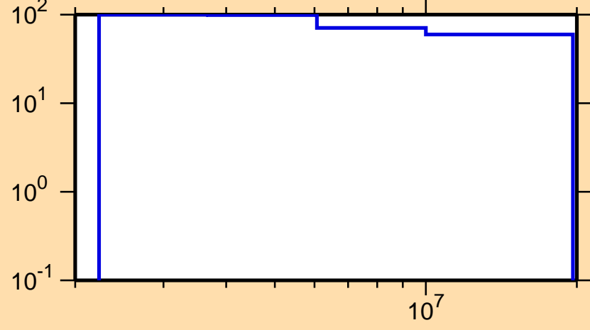
\Delta\sigma/\sigma vs. E for ^{170}\text{Os}(n,n\text{cont.})
