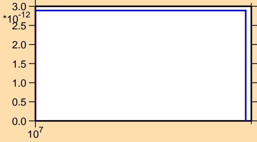
\sigma vs. E for ^{170}\text{Os} (mt 34)
