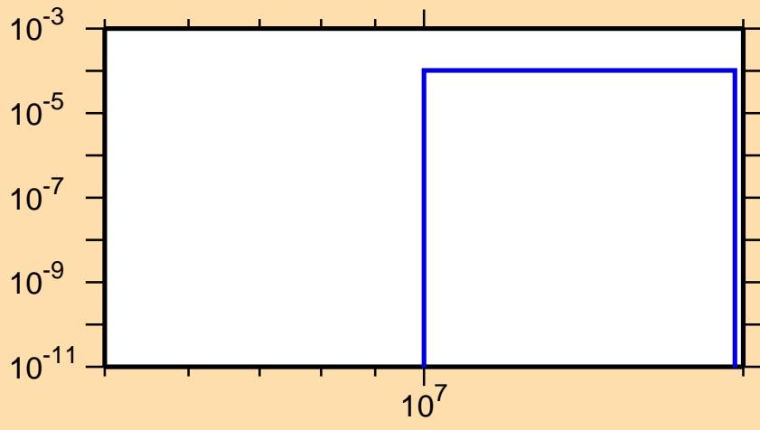
\sigma vs. E for ^{170}\text{Os}(n,2n\alpha)
