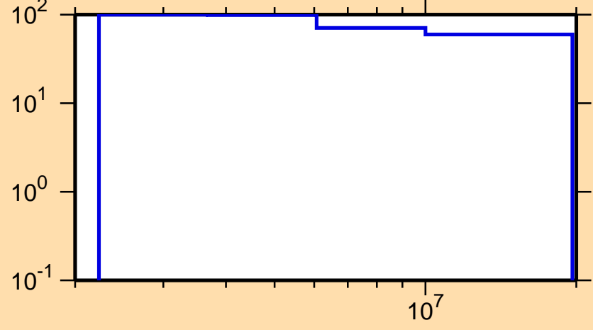
\Delta\sigma/\sigma vs. E for ^{170}\text{Os}(n,ncont.)
