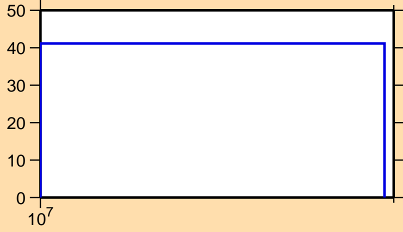
\Delta\sigma/\sigma vs. E for ^{170}\text{Os}(n,\text{inel.})
