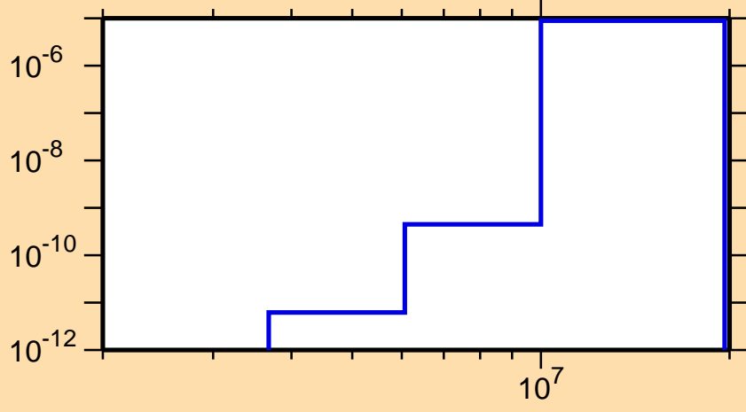
\sigma vs. E for ^{170}\text{Os}(n,\text{He}3)
