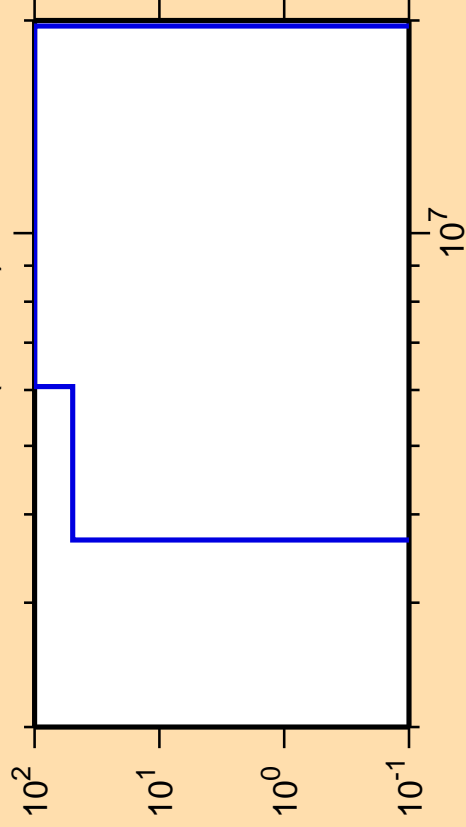
\Delta\sigma/\sigma vs. E for ^{170}\text{Os}(n,\text{He}3)
