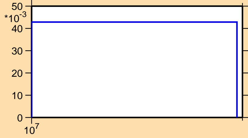
\sigma vs. E for ^{170}\text{Os}(n,2n)
