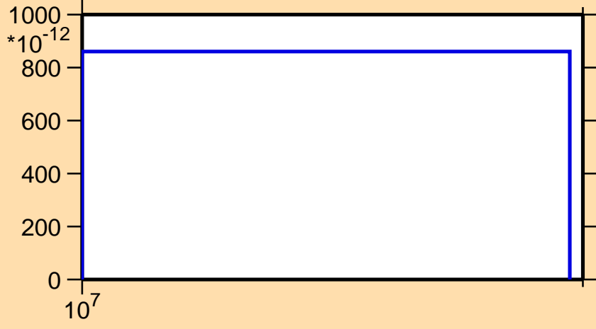
\sigma vs. E for ^{170}\text{Os}(n,\text{pt})
