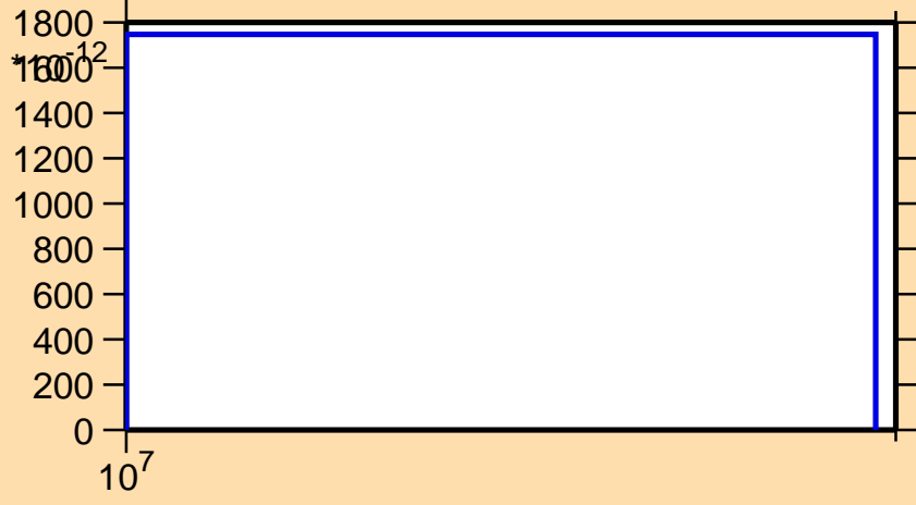
\sigma vs. E for ^{170}\text{Os}(n,\text{nd})
