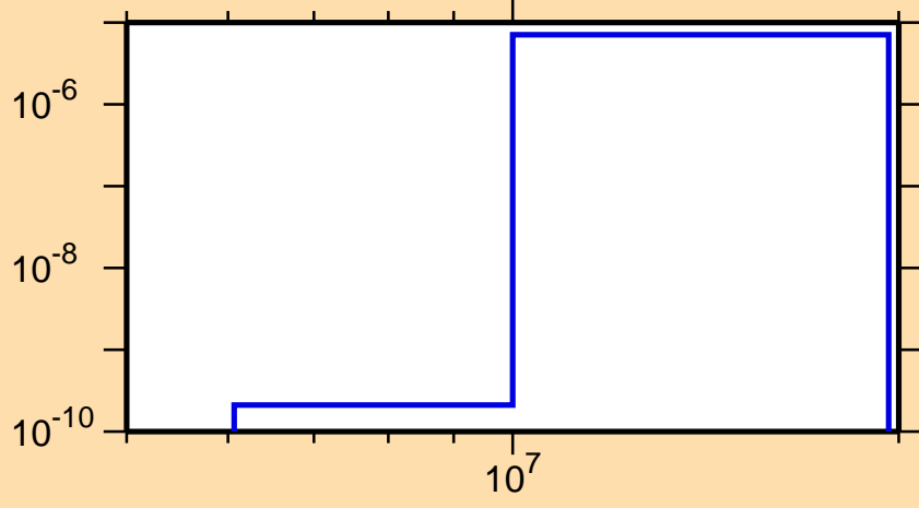
\sigma vs. E for ^{170}\text{Os} (mt 45)
