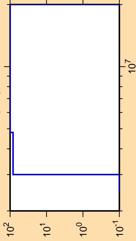
\Delta\sigma/\sigma vs. E for ^{170}\text{Os}(n,d)
