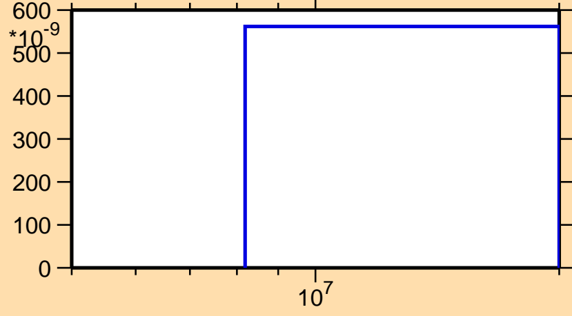
\sigma vs. E for ^{170}\text{Os}(n,2np)
