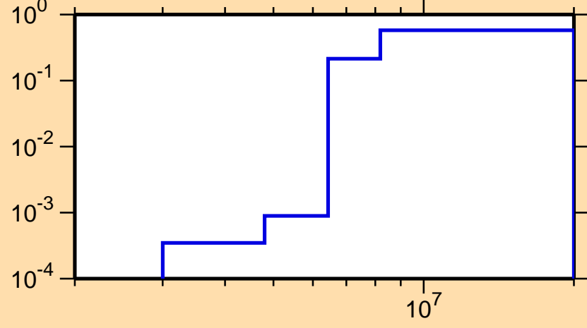
\sigma vs. E for ^{170}\text{Os}(n,n\text{cont.})
