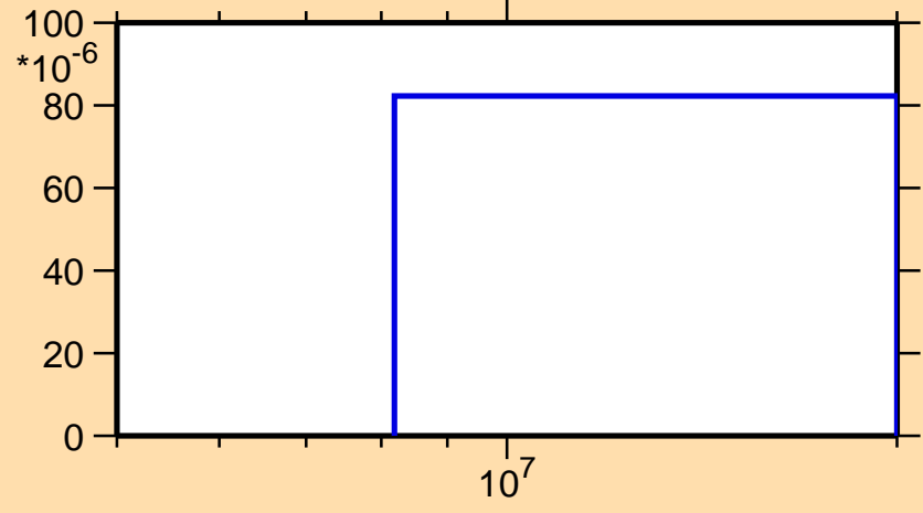
\sigma vs. E for ^{170}\text{Os}(n,2n\alpha)
