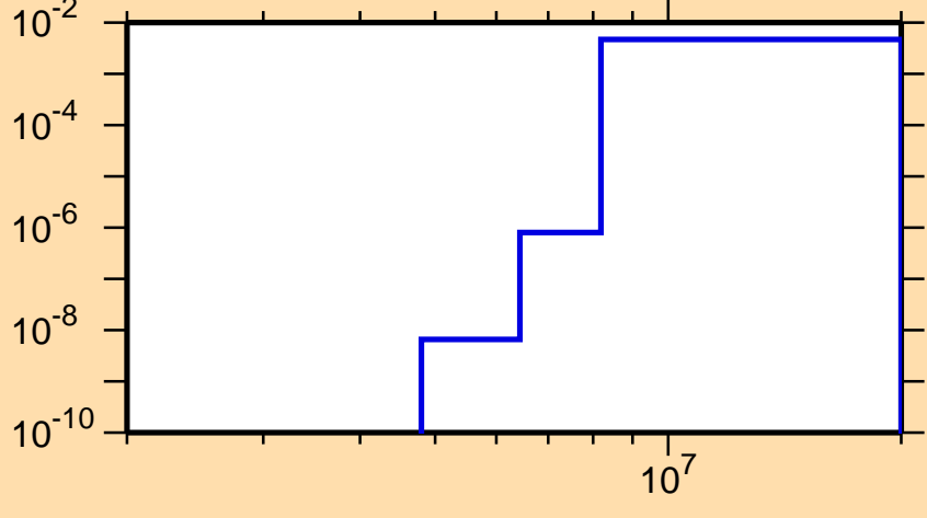
\sigma vs. E for ^{170}\text{Os}(n,d)
