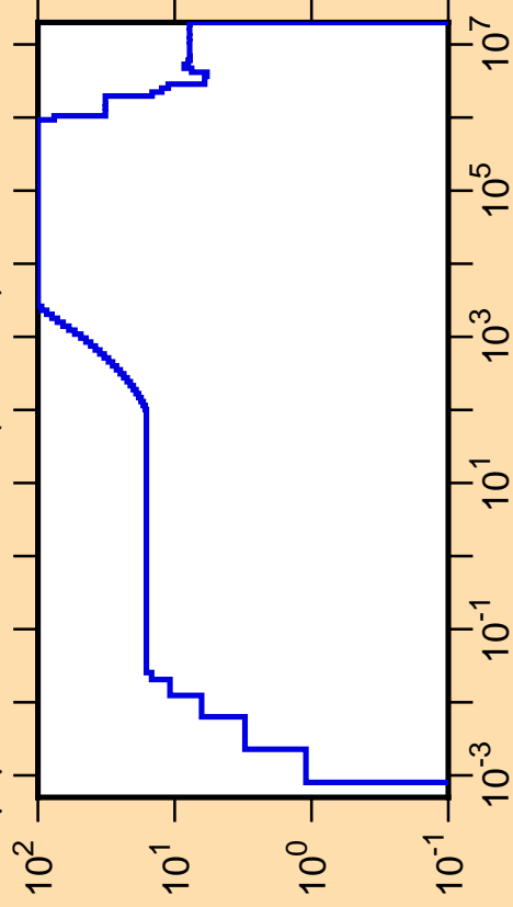
\Delta\mu/\mu vs. E for ^{171}\text{Os}(\text{mt251})
