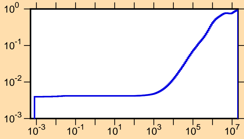
\mu vs. E for ^{171}\text{Os}(\text{mt251})
