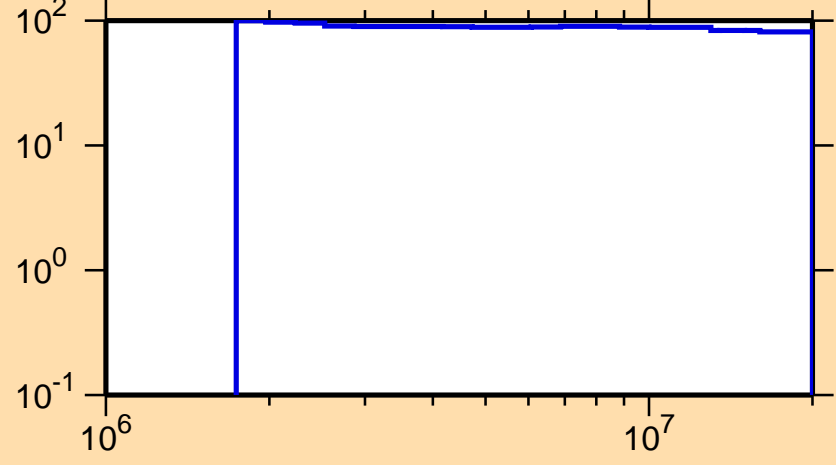
\Delta\sigma/\sigma vs. E for ^{171}\text{Os}(n,ncont.)
