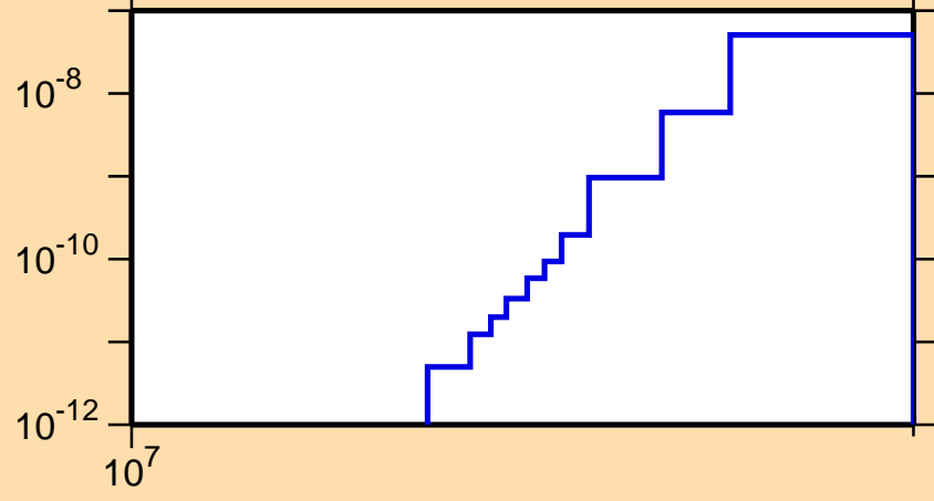
\sigma vs. E for ^{171}\text{Os} (mt 34)
