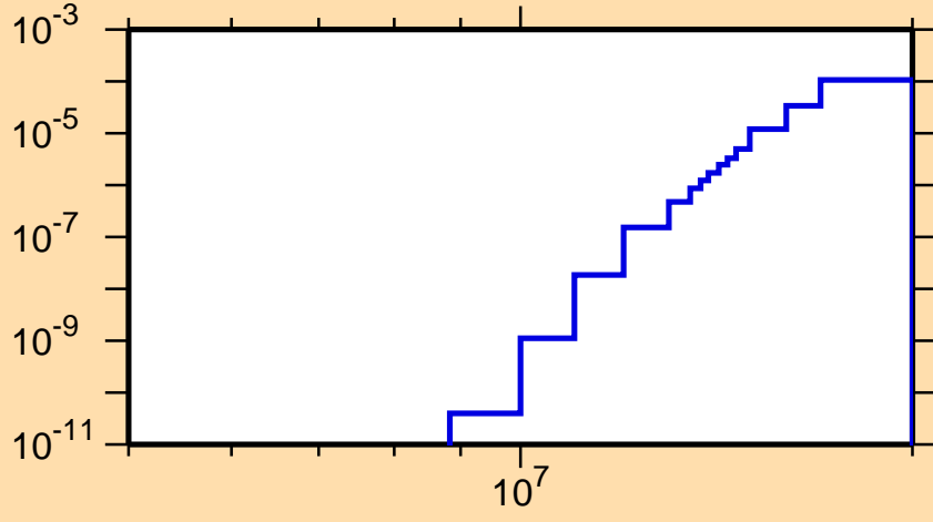
\sigma vs. E for ^{171}\text{Os} (mt 45)
