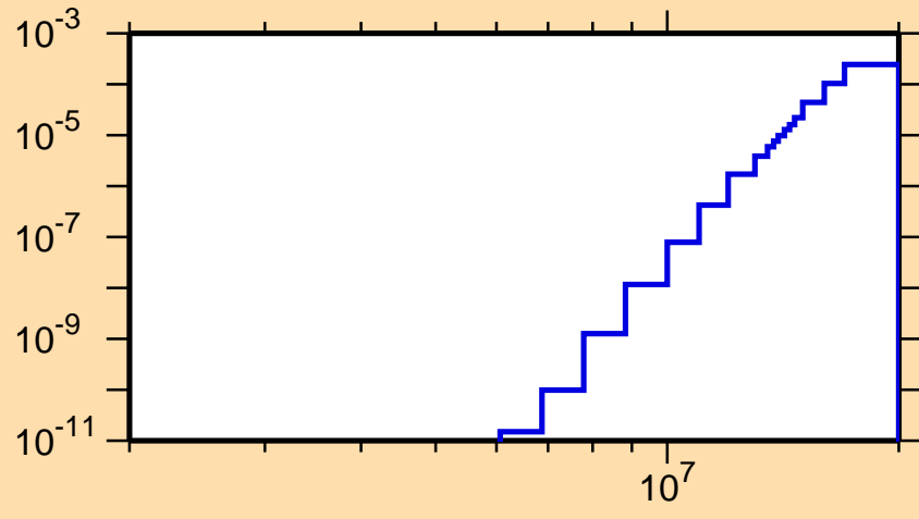
\sigma vs. E for ^{171}\text{Os}(n,\text{He}3)
