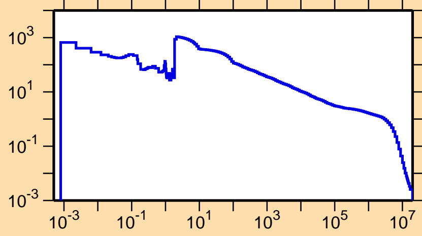
\sigma vs. E for ^{171}\text{Os}(n,\gamma)
