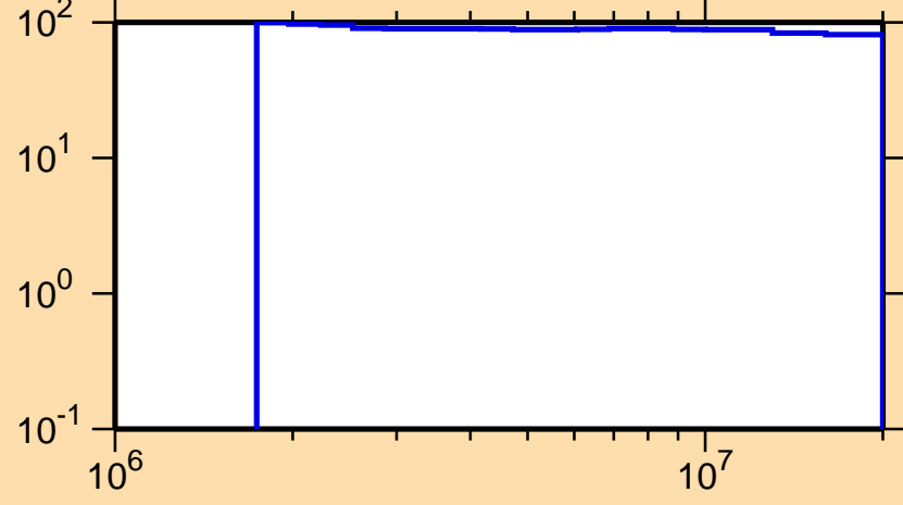
\Delta\sigma/\sigma vs. E for ^{171}\text{Os}(n,n\text{cont.})
