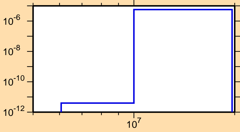
\sigma vs. E for ^{171}\text{Os} (mt 45)
