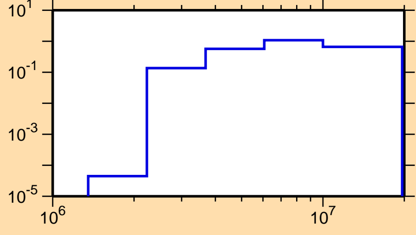
\sigma vs. E for ^{171}\text{Os}(n,n\text{cont.})
