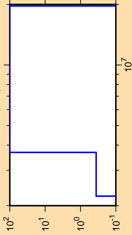
\Delta\sigma/\sigma vs. E for ^{171}\text{Os}(n,d)
