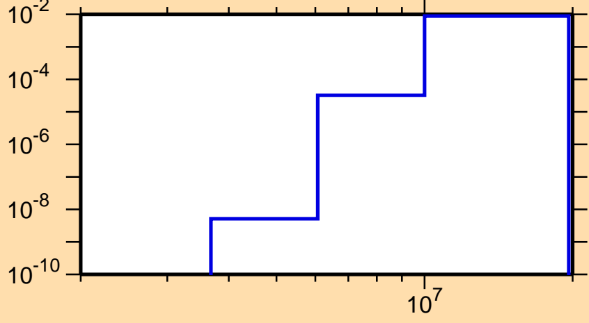
\sigma vs. E for ^{171}\text{Os}(n,d)
