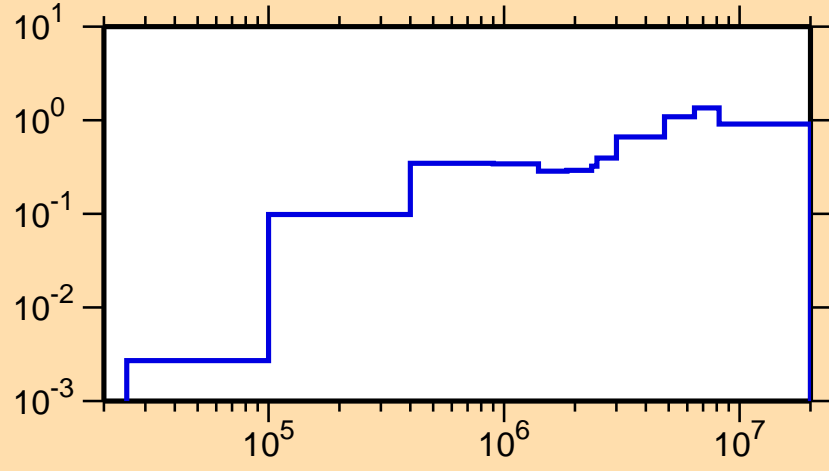
\sigma vs. E for ^{171}\text{Os}(n,\text{inel.})
