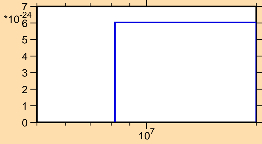
\sigma vs. E for ^{171}\text{Os}(\text{mt } 11)
