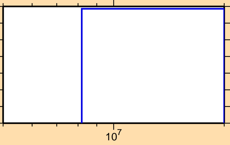
\sigma vs. E for ^{171}\text{Os}(n,\text{pt})
