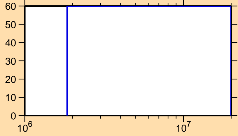
\Delta\sigma/\sigma vs. E for ^{171}\text{Os}(n,ncont.)
