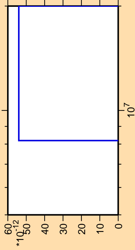
\Delta\sigma/\sigma vs. E for ^{171}\text{Os}(\text{mt } 11)
