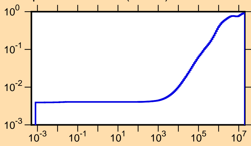
\mu vs. E for ^{172}\text{Os}(\text{mt251})
