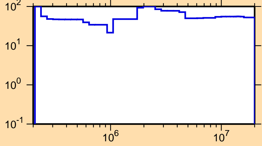
\Delta\sigma/\sigma vs. E for ^{172}\text{Os}(n,n_1)
