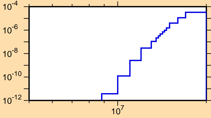
\sigma vs. E for ^{172}\text{Os} (mt 45)
