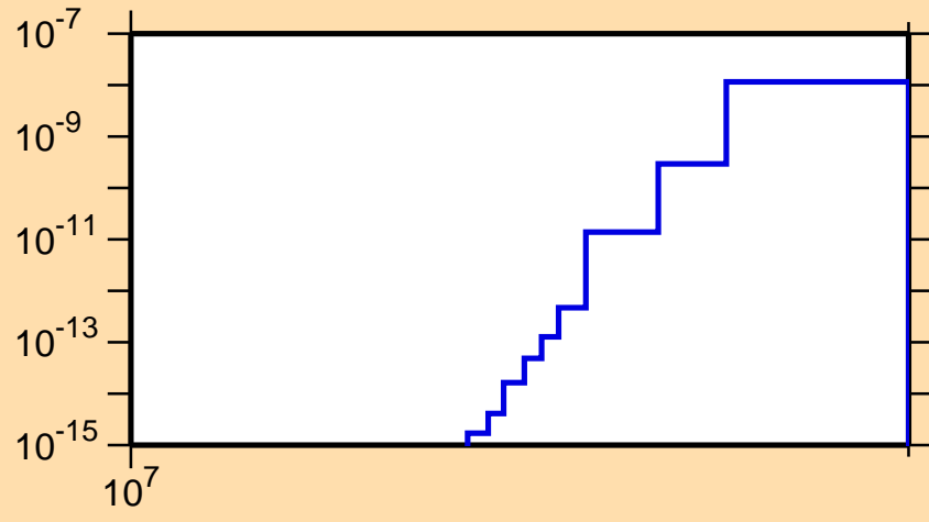
\sigma vs. E for ^{172}\text{Os}(n,\text{pt})
