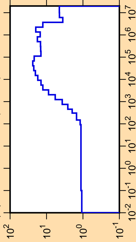
\Delta\mu/\mu vs. E for ^{172}\text{Os}(\text{mt251})
