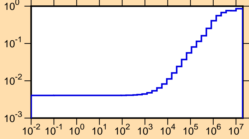
\mu vs. E for ^{172}\text{Os}(\text{mt251})
