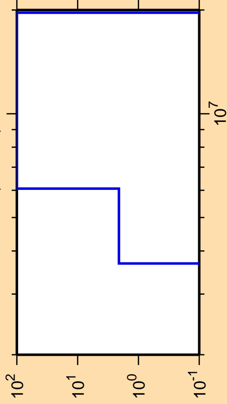
\Delta\sigma/\sigma vs. E for ^{172}\text{Os}(n,\text{He3})
