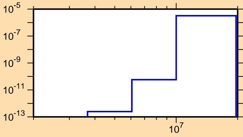
\sigma vs. E for ^{172}\text{Os}(n,\text{He3})
