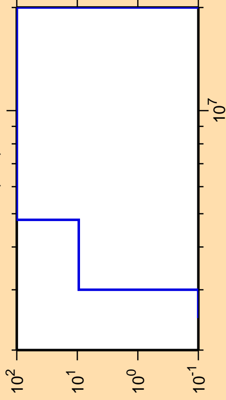
\Delta\sigma/\sigma vs. E for ^{172}\text{Os}(n,d)
