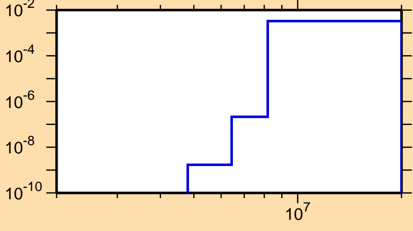
\sigma vs. E for ^{172}\text{Os}(n,d)
