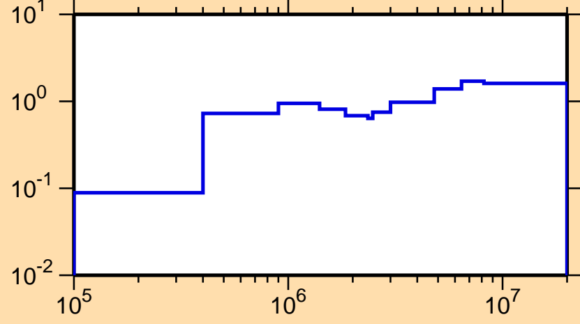
\sigma vs. E for ^{172}\text{Os}(n,\text{inel.})
