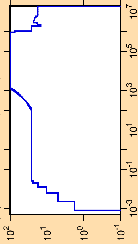
\Delta\mu/\mu vs. E for ^{173}\text{Os}(\text{mt251})
