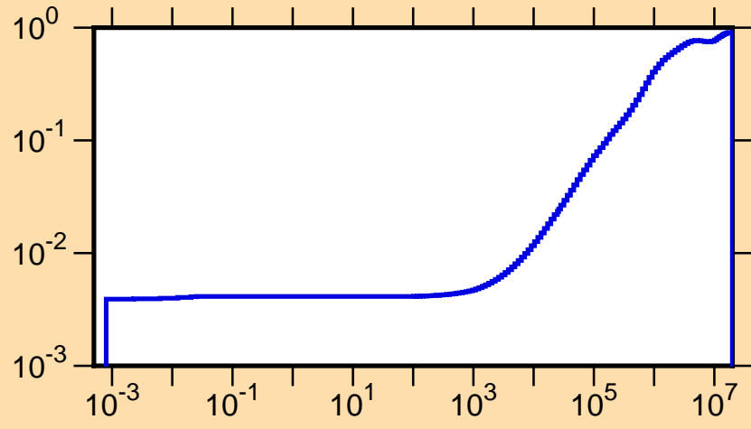
\mu vs. E for ^{173}\text{Os}(\text{mt251})
