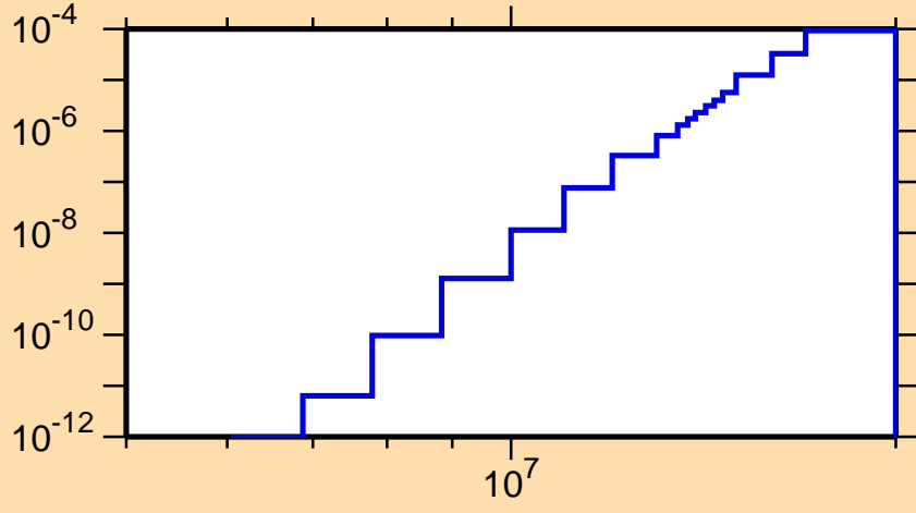
\sigma vs. E for ^{173}\text{Os}(n,\text{He3})
