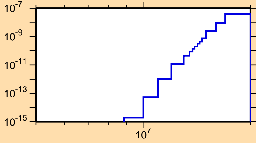
\sigma vs. E for ^{173}\text{Os} (mt117)
