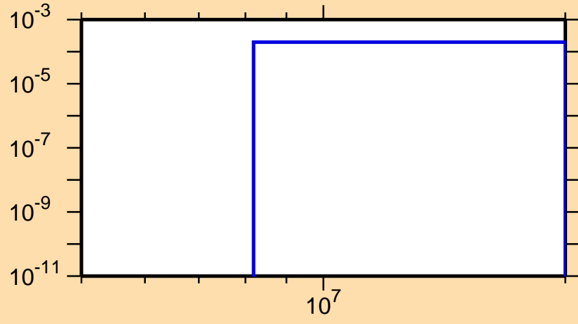
\sigma vs. E for ^{173}\text{Os}(n,t)
