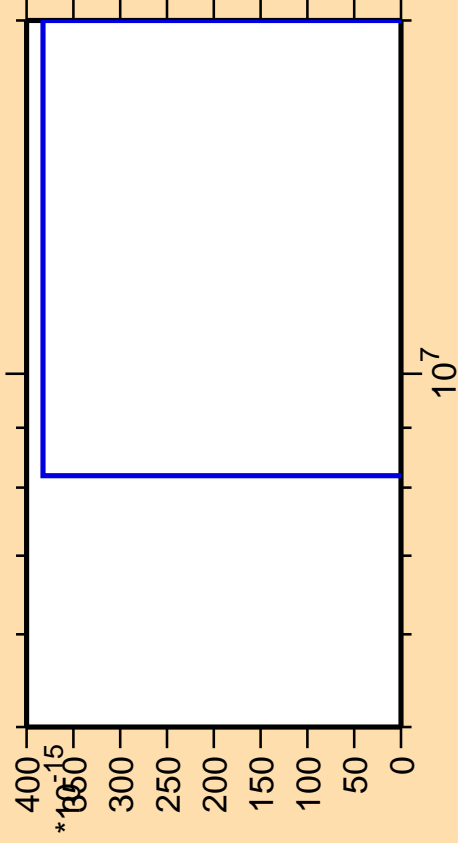
\Delta\sigma/\sigma vs. E for ^{173}\text{Os}(\text{mt 11})
