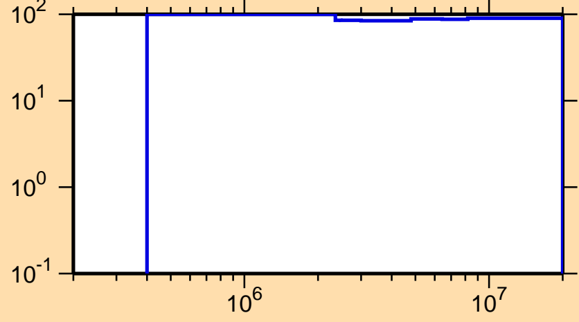
\Delta\sigma/\sigma vs. E for ^{173}\text{Os}(n,ncont.)
