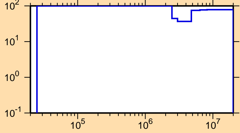
\Delta\sigma/\sigma vs. E for ^{173}\text{Os}(n,\text{inel.})
