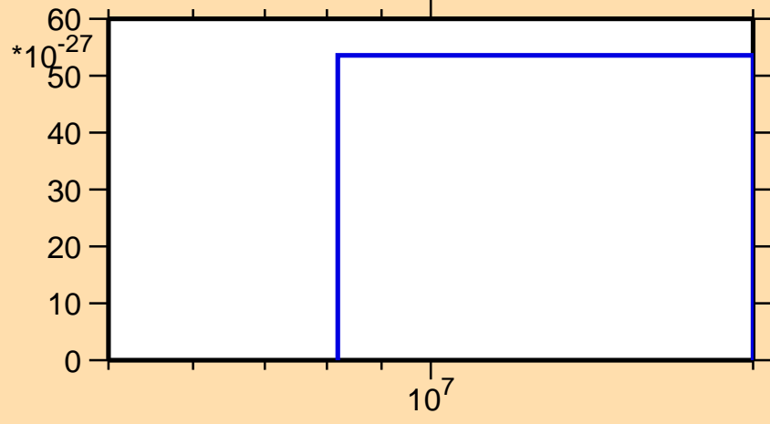
\sigma vs. E for ^{173}\text{Os}(\text{mt 11})
