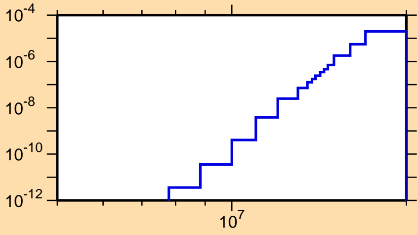
\sigma vs. E for ^{174}\text{Os}(n,\text{He3})
