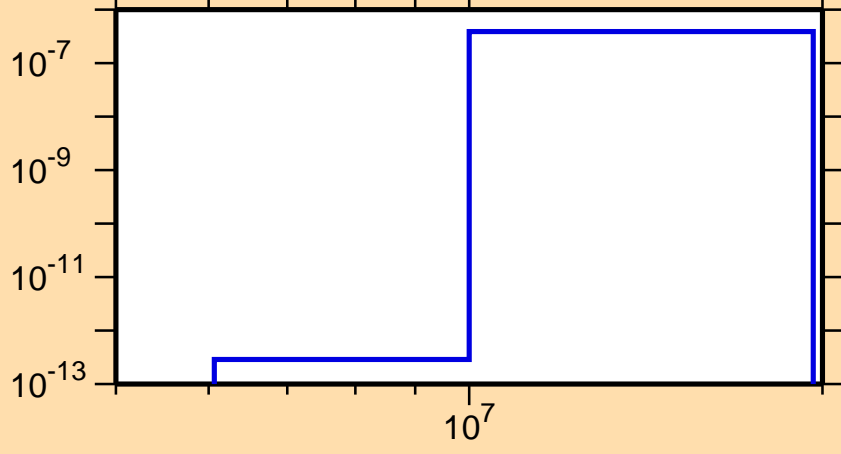
\sigma vs. E for ^{174}\text{Os}(n,2n\alpha)
