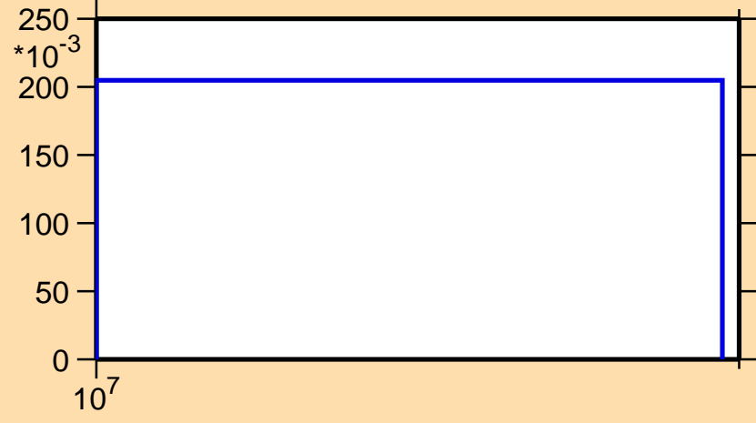
\sigma vs. E for ^{174}\text{Os}(n,2n)
