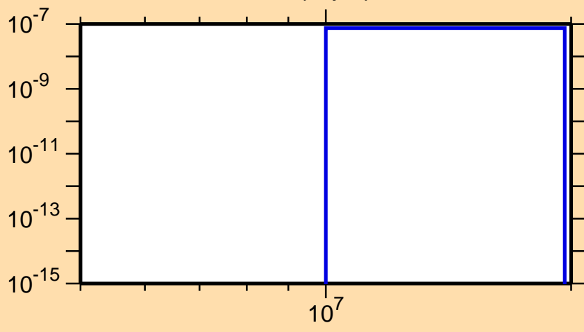
\sigma vs. E for ^{174}\text{Os}(n,\text{pd})
