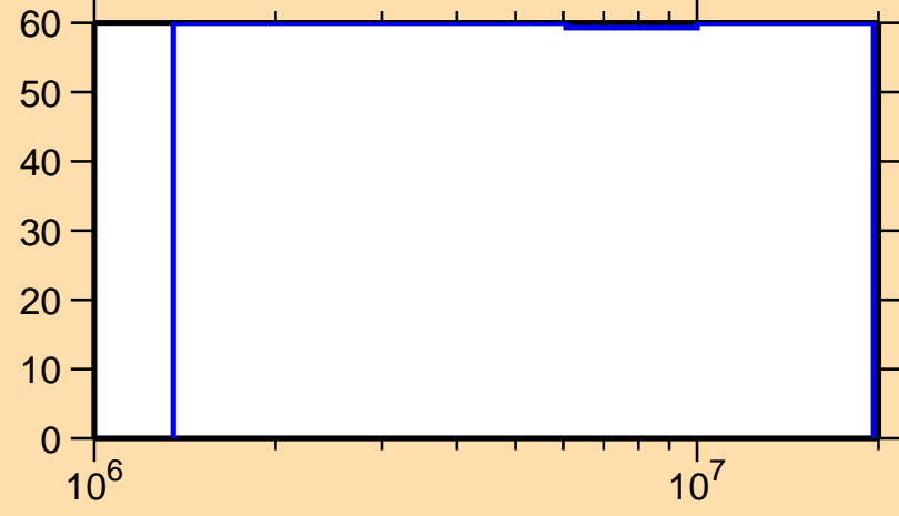
\Delta\sigma/\sigma vs. E for ^{174}\text{Os}(n,n\text{cont.})
