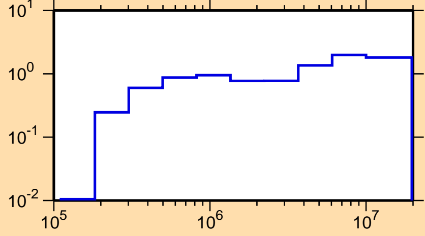
\sigma vs. E for ^{174}\text{Os}(n,\text{inel.})
