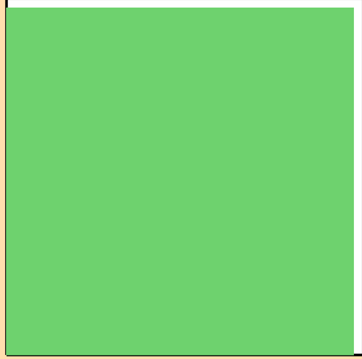
\Delta\sigma/\sigma vs. E for ^{174}\text{Os}(n,2n)
