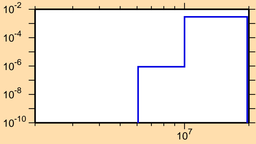
\sigma vs. E for ^{174}\text{Os}(n,d)
