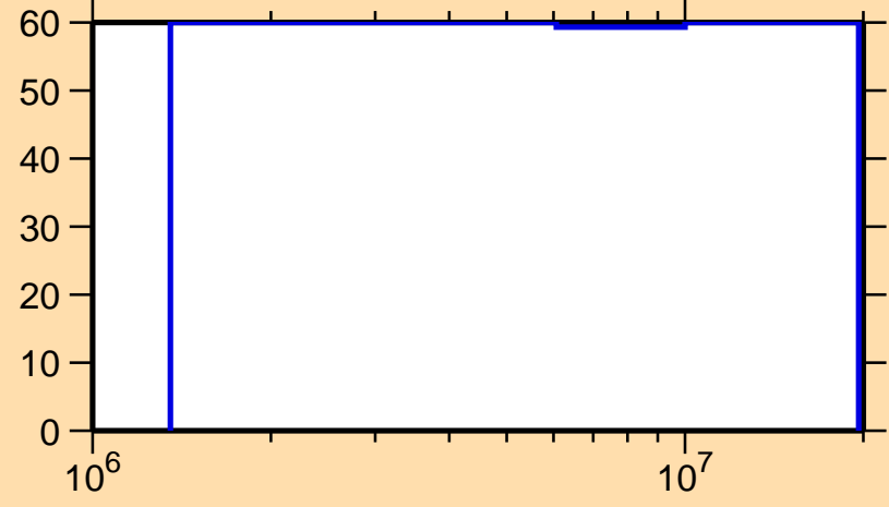
\Delta\sigma/\sigma vs. E for ^{174}\text{Os}(n,ncont.)
