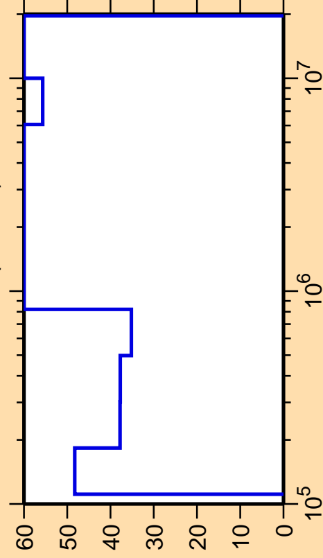
\Delta\sigma/\sigma vs. E for ^{174}\text{Os}(n,\text{inel.})
