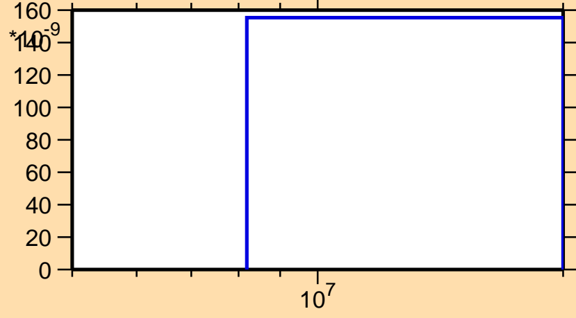
\sigma vs. E for ^{174}\text{Os}(n,2np)
