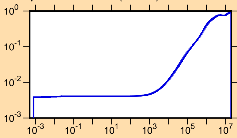
\mu vs. E for ^{175}\text{Os}(\text{mt251})
