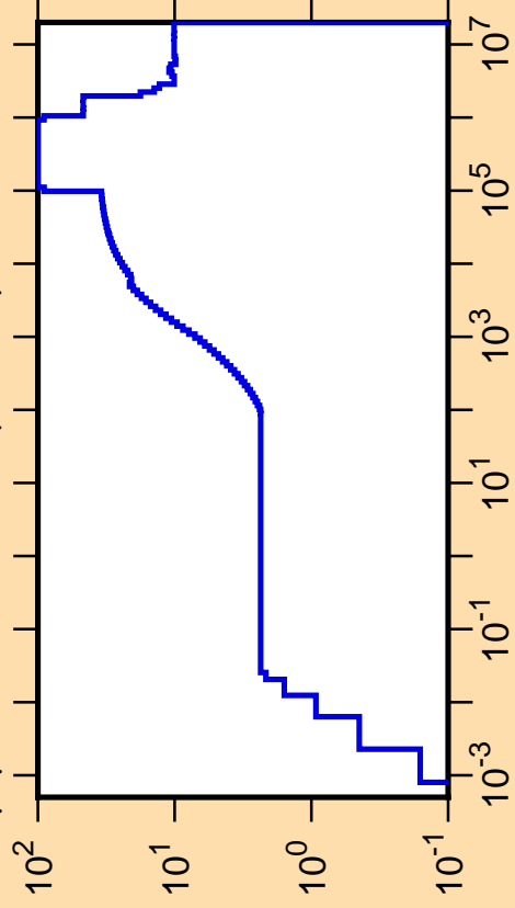
\Delta\mu/\mu vs. E for ^{175}\text{Os}(\text{mt251})
