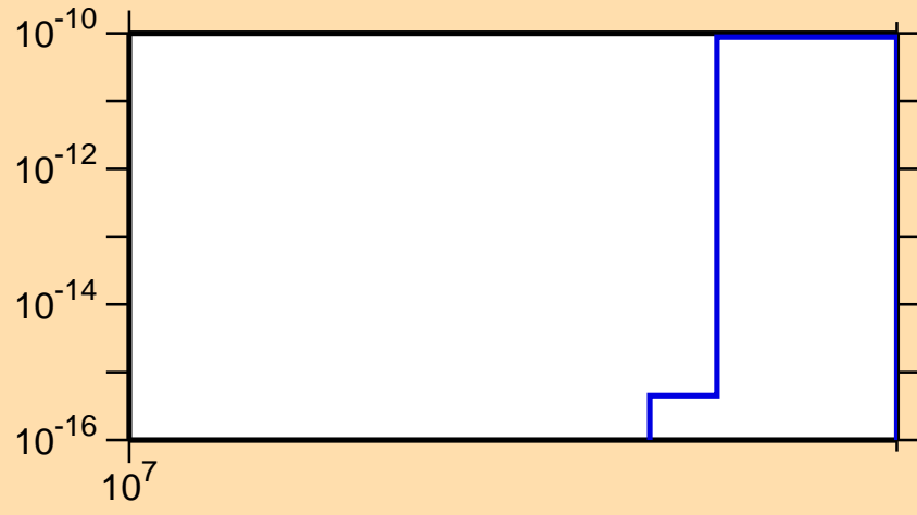
\sigma vs. E for ^{175}\text{Os}(n,nt)
