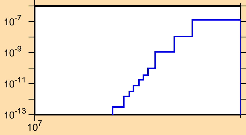
\sigma vs. E for ^{175}\text{Os}(n,pt)
