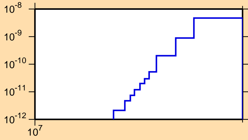
\sigma vs. E for ^{175}\text{Os}(\text{mt117})
