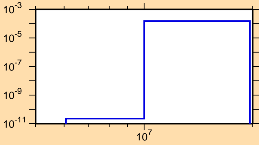
\sigma vs. E for ^{175}\text{Os}(n,t)
