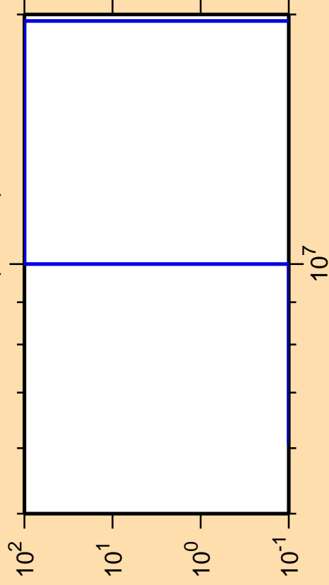
\Delta\sigma/\sigma vs. E for ^{175}\text{Os}(\text{mt } 45)
