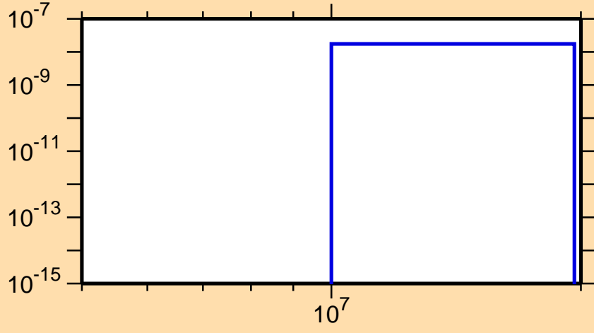
\sigma vs. E for ^{175}\text{Os}(\text{mt } 45)
