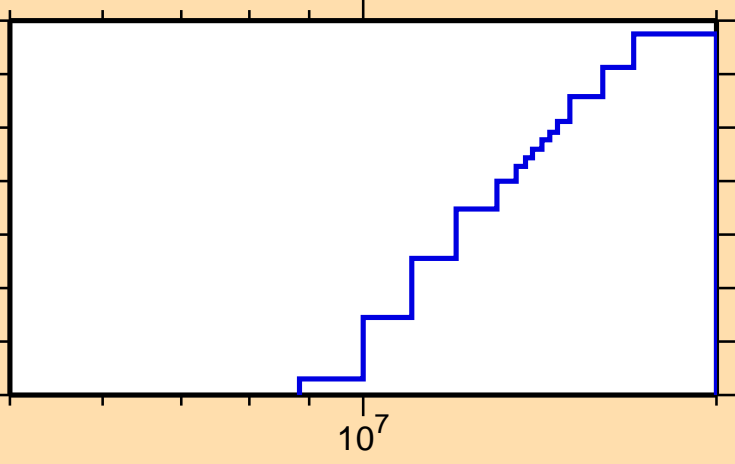
\sigma vs. E for ^{176}\text{Os}(n,\text{He3})
