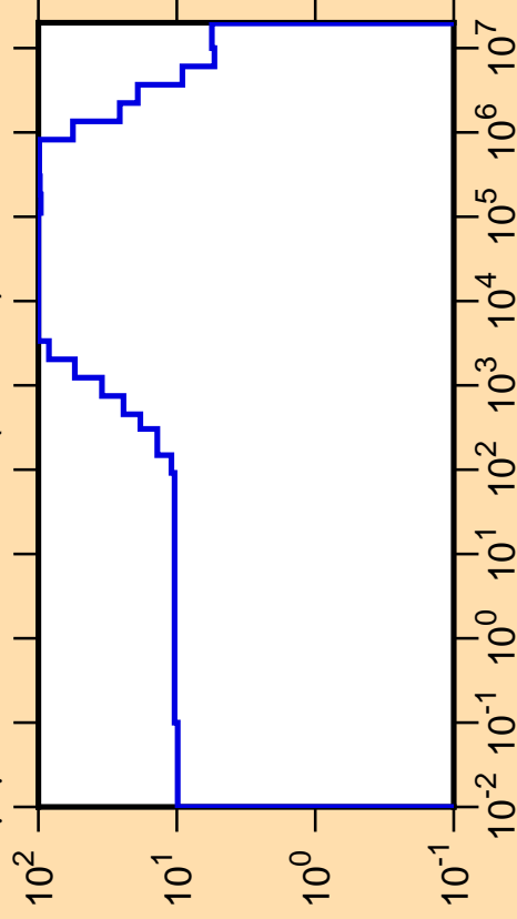
\Delta\mu/\mu vs. E for ^{176}\text{Os}(\text{mt251})
