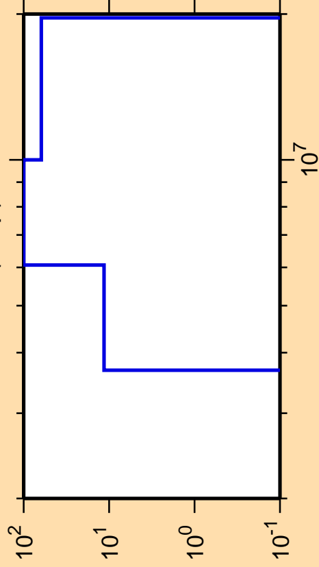
\Delta\sigma/\sigma vs. E for ^{176}\text{Os}(n,np)
