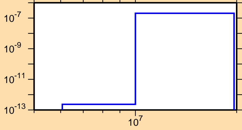
\sigma vs. E for ^{176}\text{Os}(n,\text{He}3)
