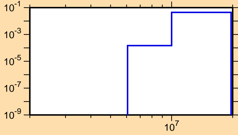
\sigma vs. E for ^{176}\text{Os}(n,np)
