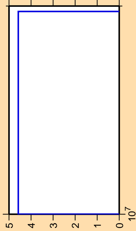
\Delta\sigma/\sigma vs. E for ^{176}\text{Os}(n,\text{pt})
