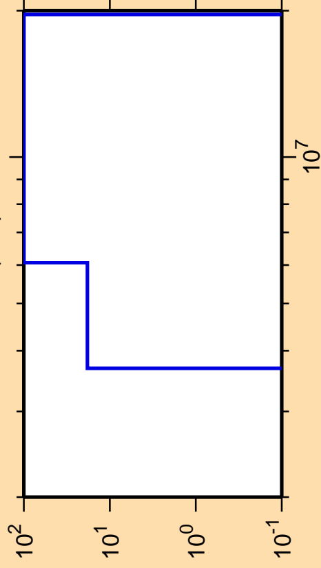
\Delta\sigma/\sigma vs. E for ^{176}\text{Os}(n,d)
