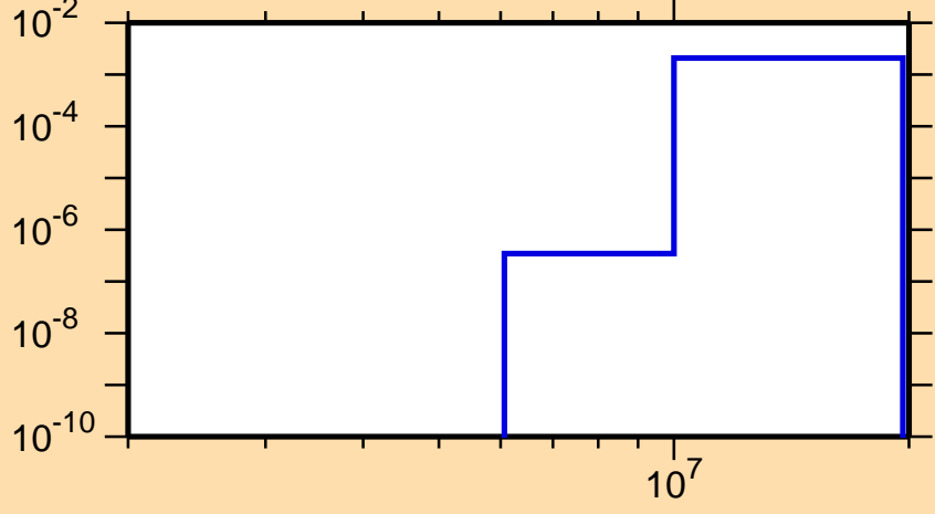
\sigma vs. E for ^{176}\text{Os}(n,d)
