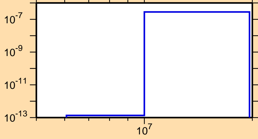
\sigma vs. E for ^{176}\text{Os}(n,2n\alpha)
