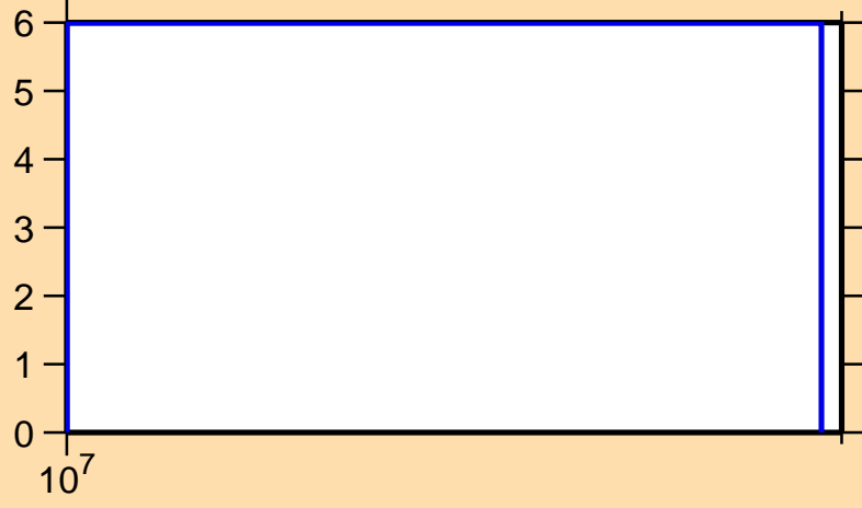
\Delta\sigma/\sigma vs. E for ^{176}\text{Os}(n,\text{nonel.})
