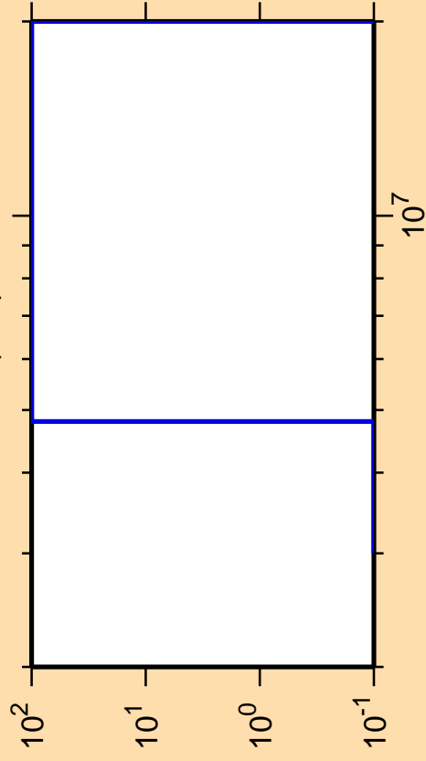
\Delta\sigma/\sigma vs. E for ^{176}\text{Os}(n,d)
