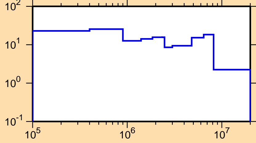
\Delta\sigma/\sigma vs. E for ^{176}\text{Os}(n,\text{tot.})
