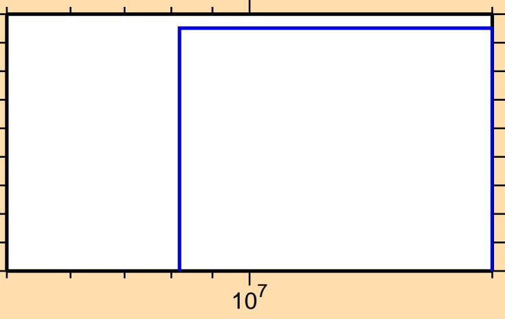
\sigma vs. E for ^{176}\text{Os}(n,3n)
