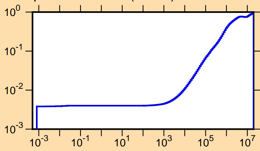
\mu vs. E for ^{177}\text{Os}(\text{mt251})
