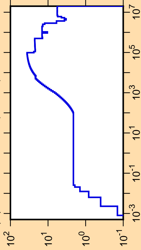
\Delta\mu/\mu vs. E for ^{177}\text{Os}(\text{mt251})
